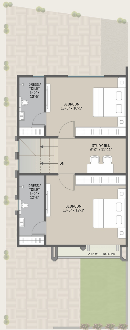
FIRST FLOOR
