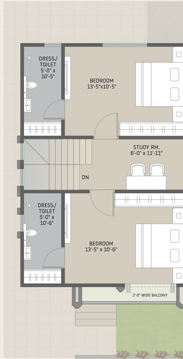
FIRST FLOOR
