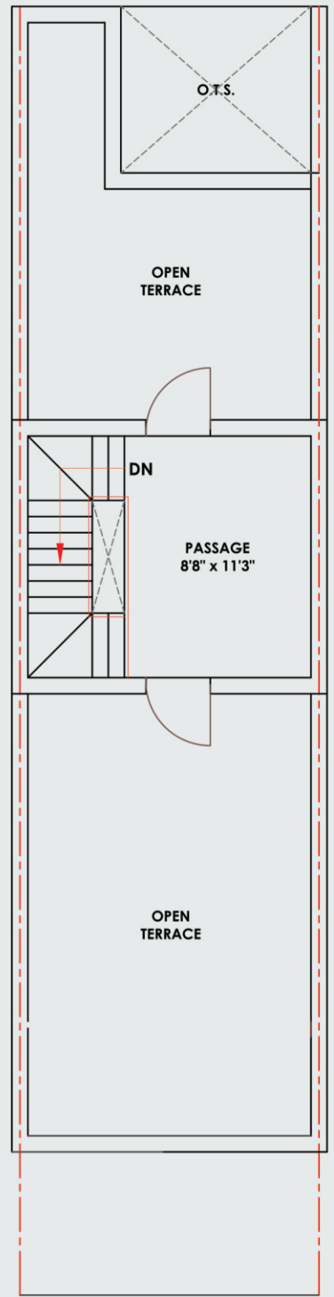
TERRACE PLAN
