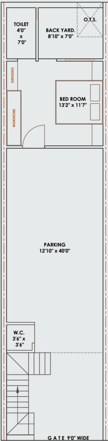
.....7.50 mt. WIDE ROAD..... GROUND FLOOR PLAN
