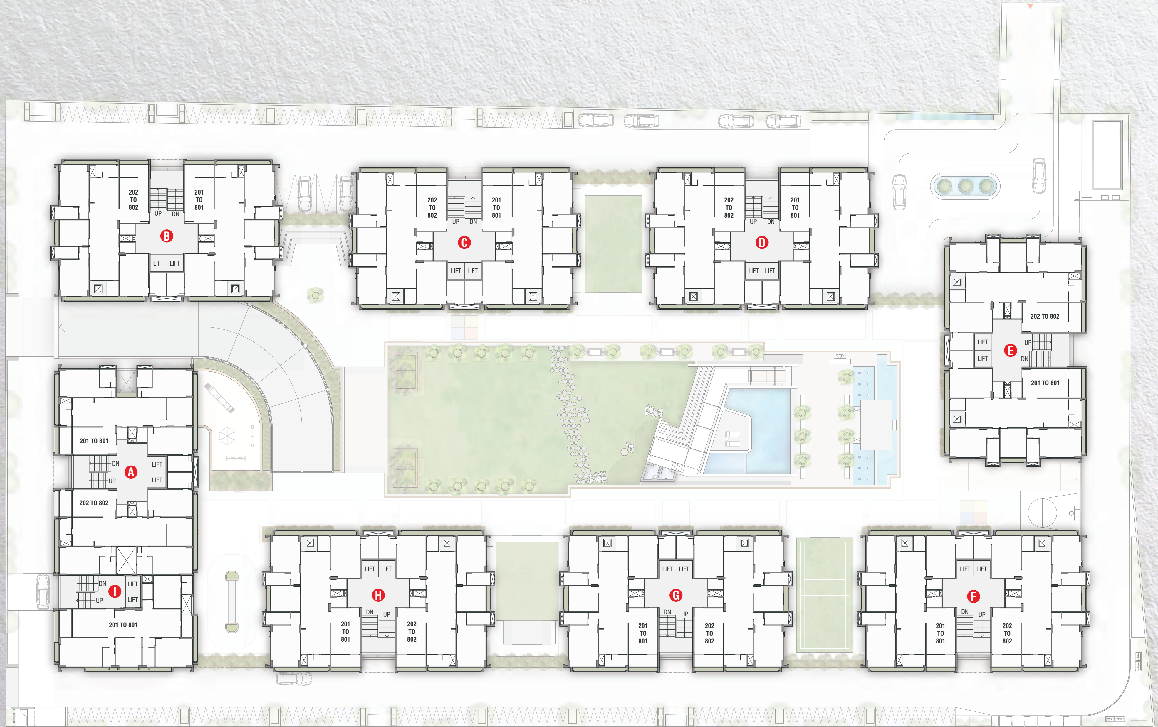
TYPICAL FLOOR LAYOUT
