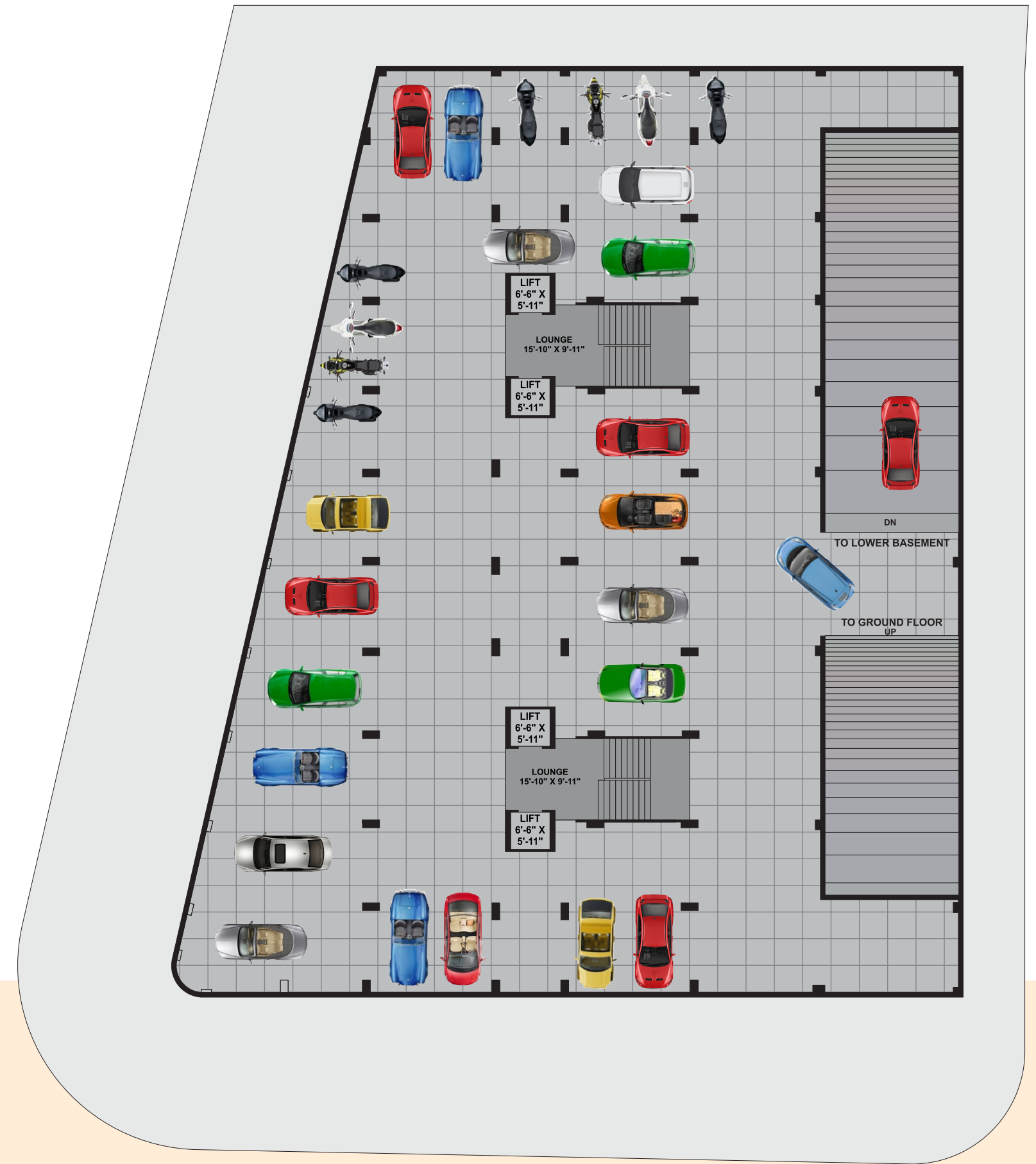
UPPER BASEMENT FLOOR
