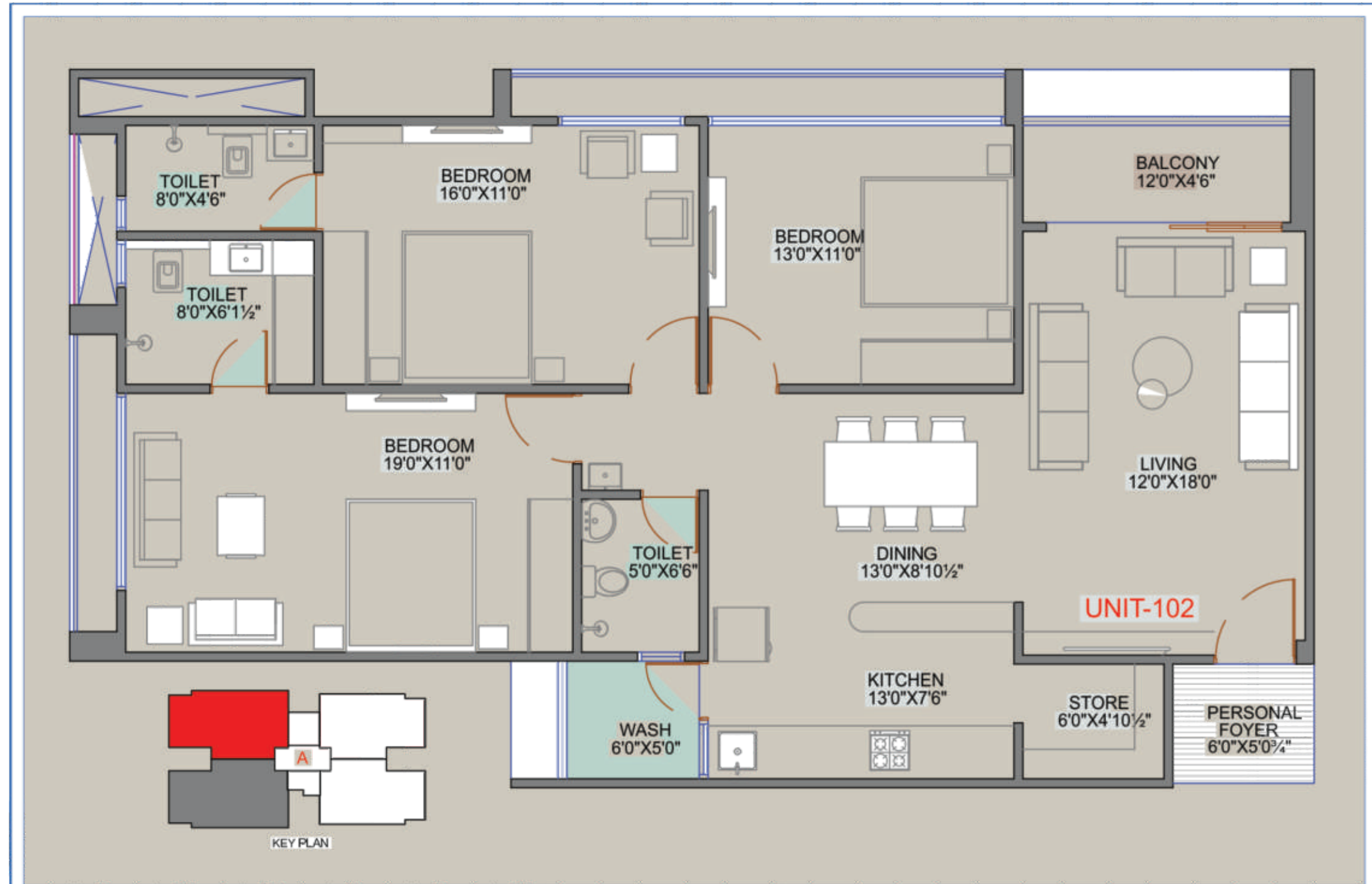
TYPICAL UNIT PLAN BLOCK -A (UNIT - 102) 28 IVY @ CHHARODI, AHMEDABAD 06 DEVELOPED BY KALPVUKSH INFRASTRUCTURE N 312, WEST FACE, opp Turban Restaurant, Nr baghian Pasty Plot, Thaltej Hebatpur Rd, Thaltej, ABAD-380060 Mob: +91 98013 30610 Email: dipacharya09@gmail.com
