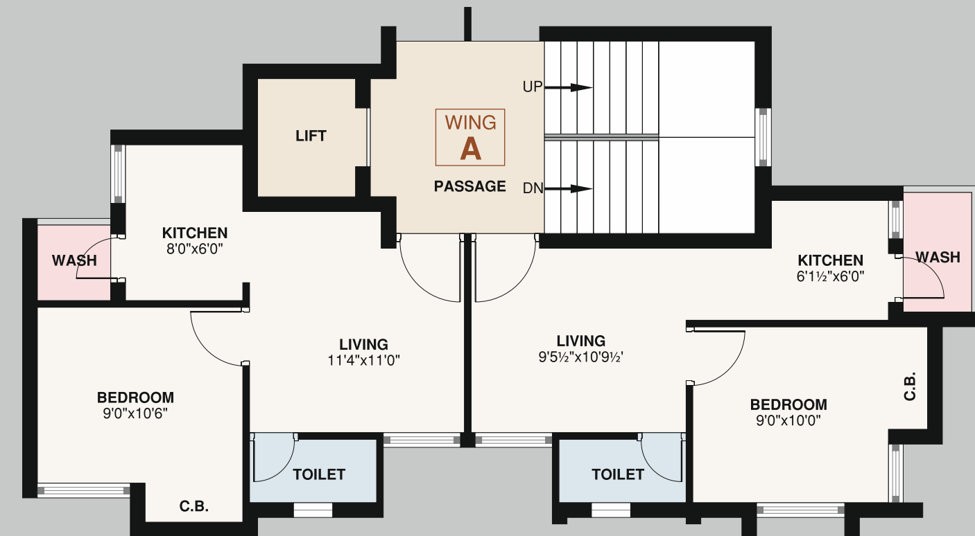
UNIT PLAN
