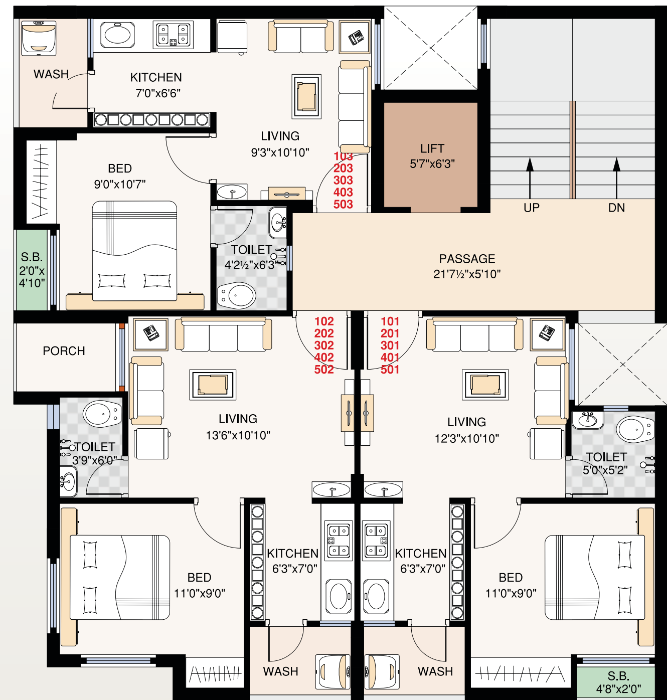
FIRST TO FIFTH FLOOR PLAN
