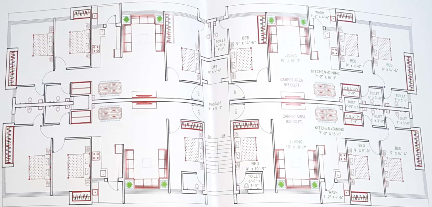
Typical 1st to 5th Floor Plan
