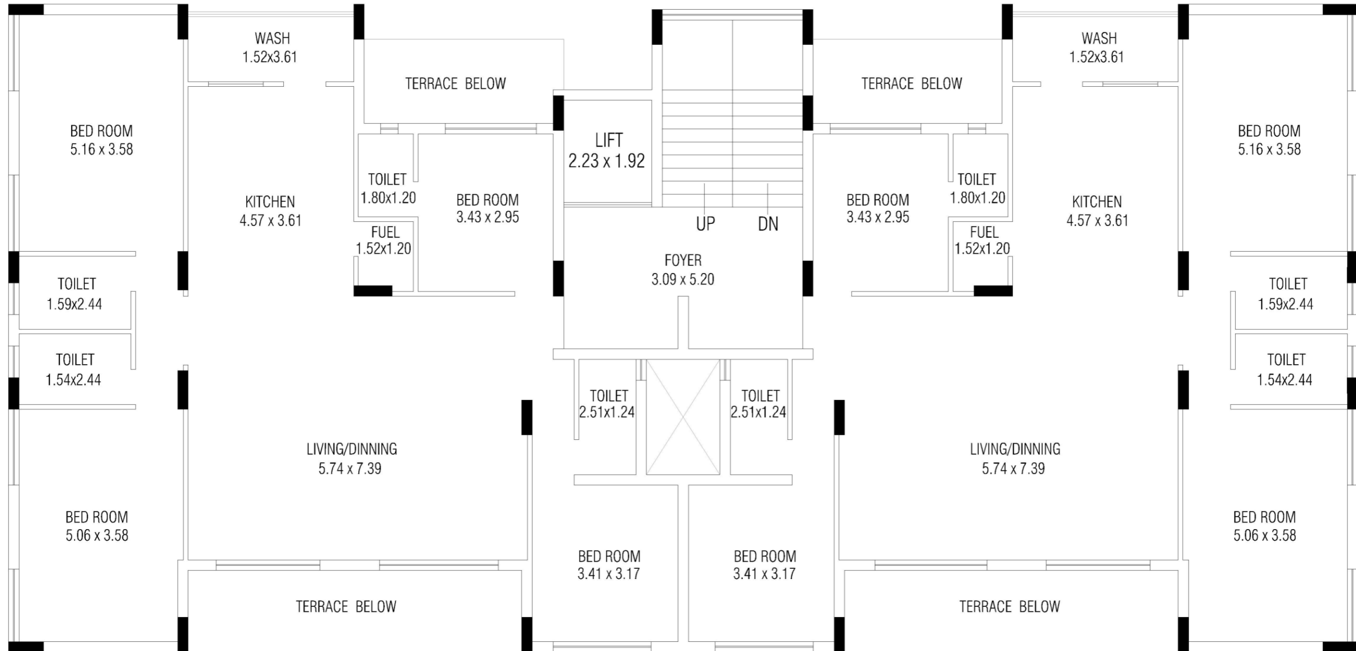
1st to 7th TYPICAL FLOOR PLAN
