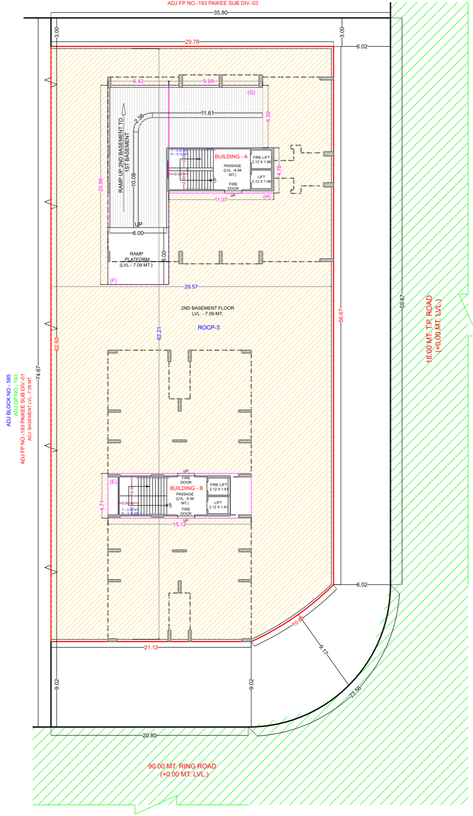
2ND BASEMENT FLOOR PLAN
