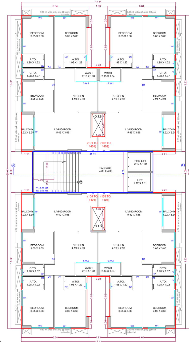
BUILDING :- 'B' TYPICAL FLOOR (1ST TO 14TH FLOOR)
