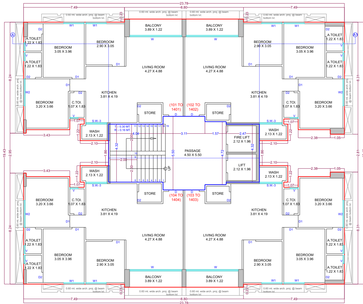
BUILDING :- 'A' TYPICAL FLOOR (1ST TO 14TH FLOOR)
