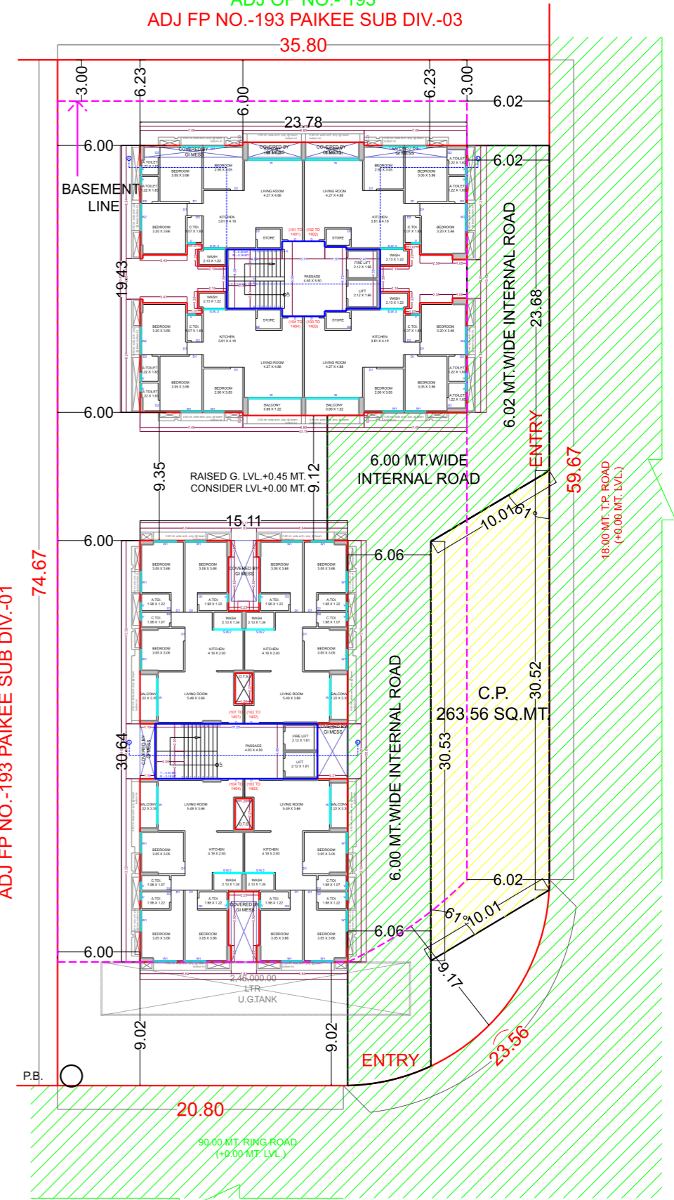
TYPICAL FLOOR PLAN [1ST TO 14TH FLOOR PLAN]
