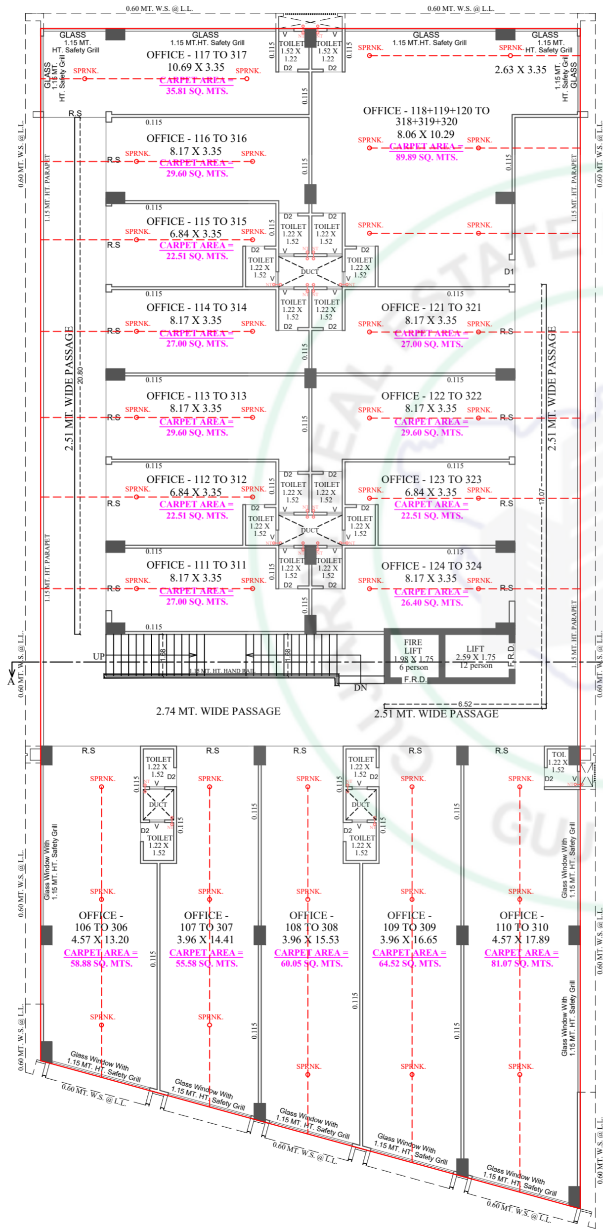
1ST TO 3RD FLOOR PLAN
