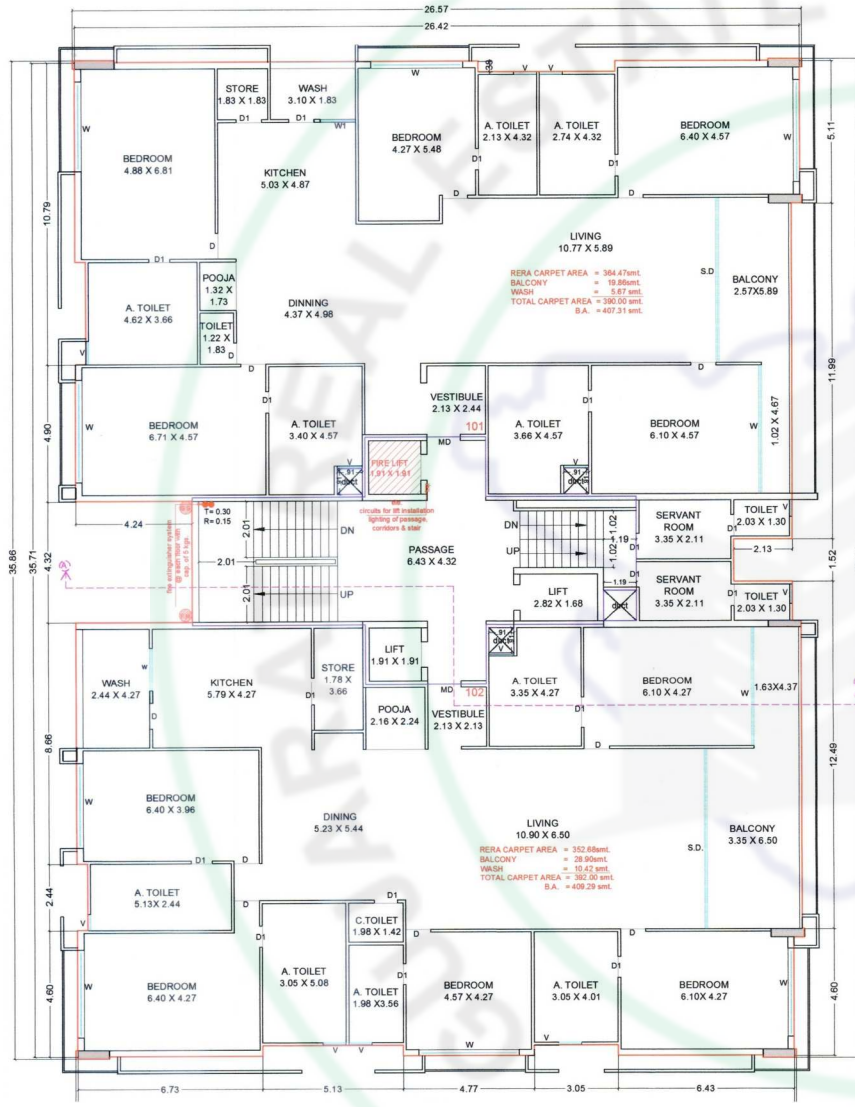
TYPICAL FLOOR PLAN (1ST TO 12TH)
