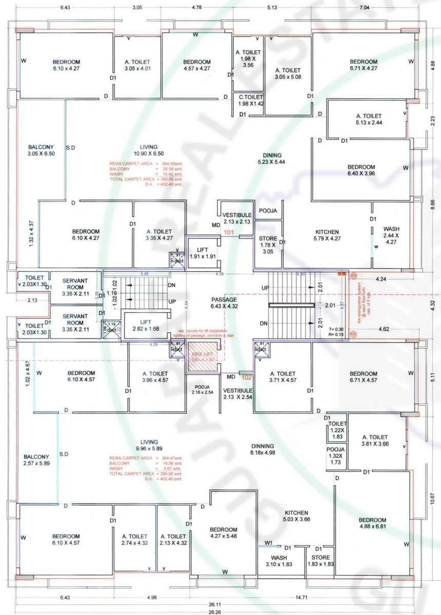
TYPICAL FLOOR PLAN (1ST TO 12TH)
