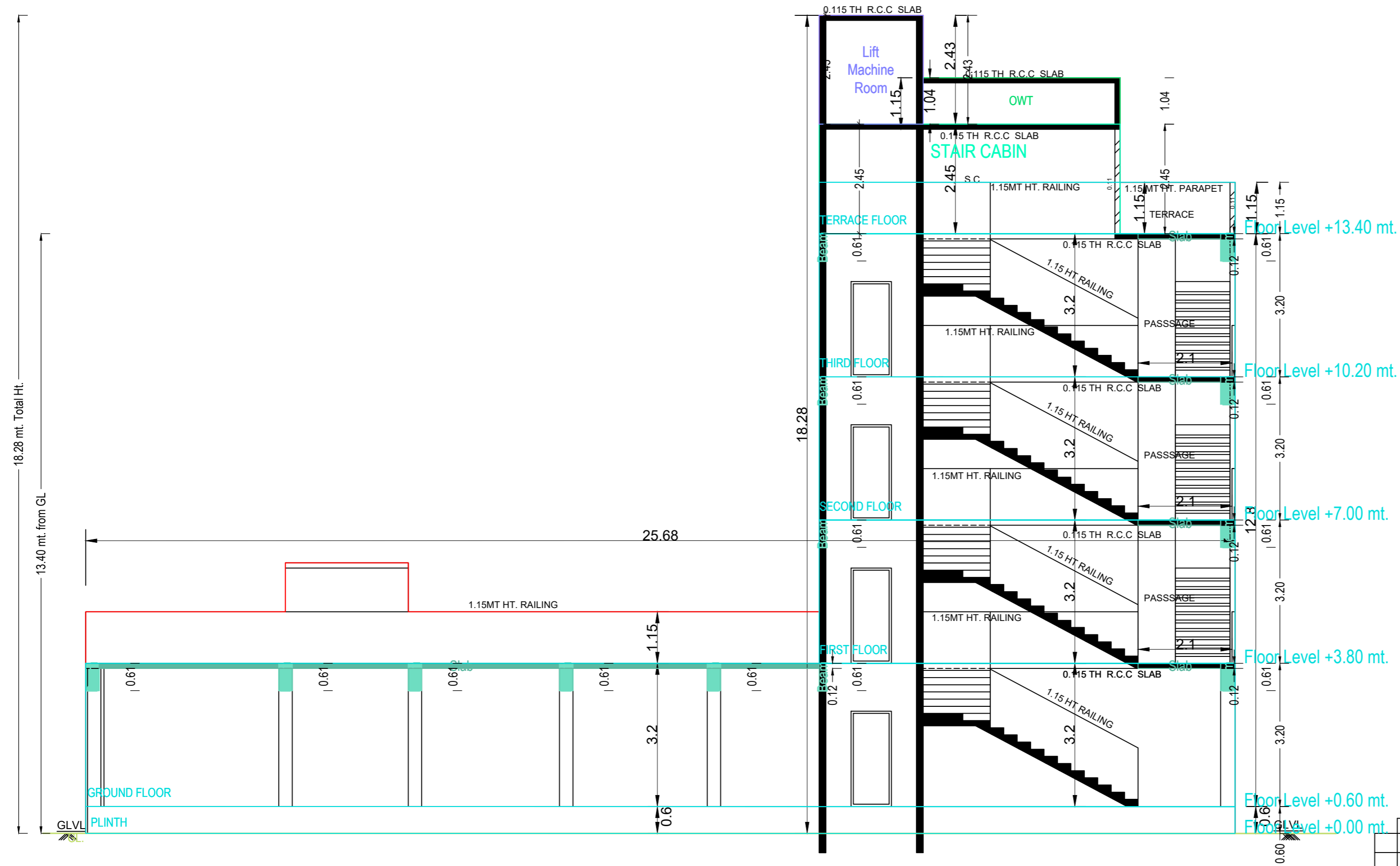
SECTION-A-A
