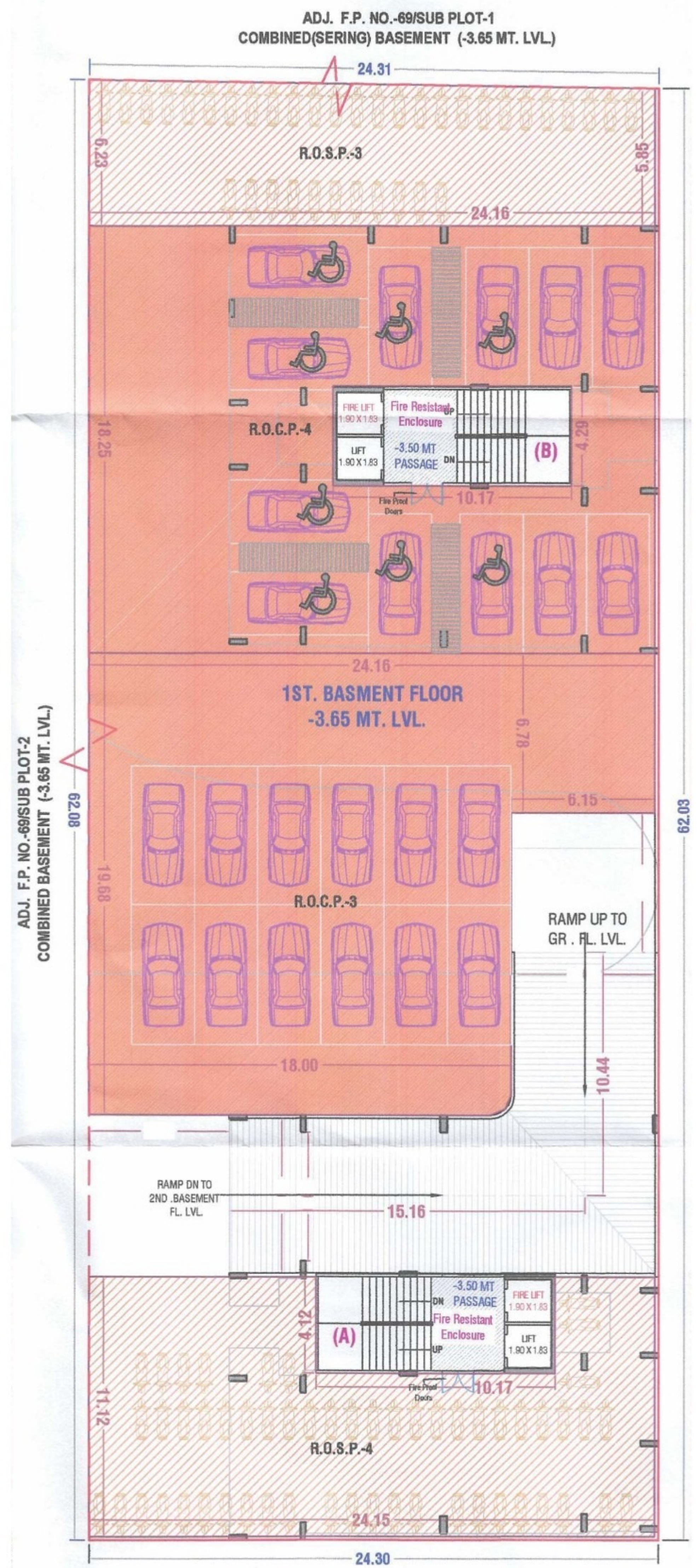
1st BASEMENT PLAN
