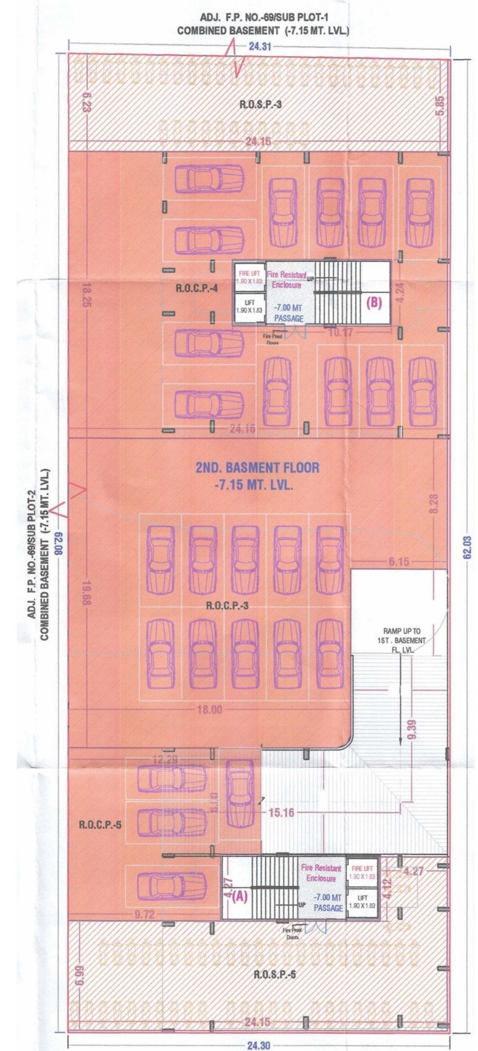
2nd BASEMENT PLAN
