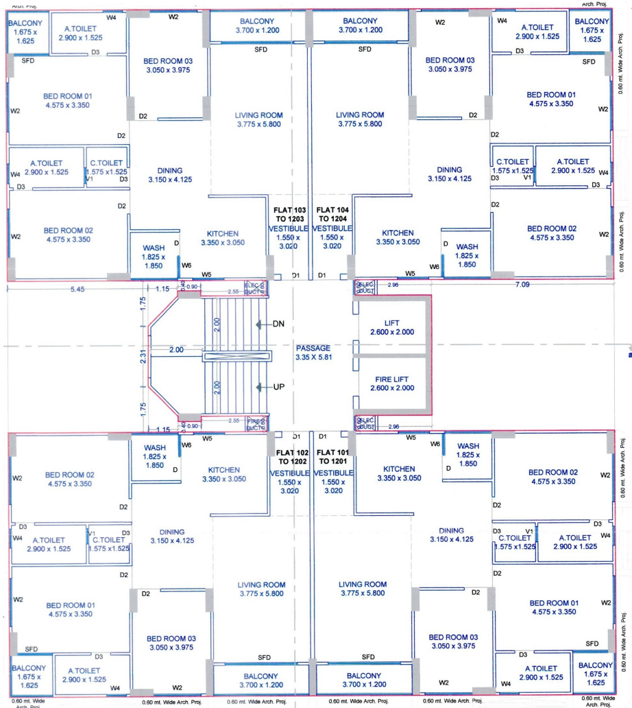
TYPICAL FLOOR PLAN (1ST TO 12TH)
