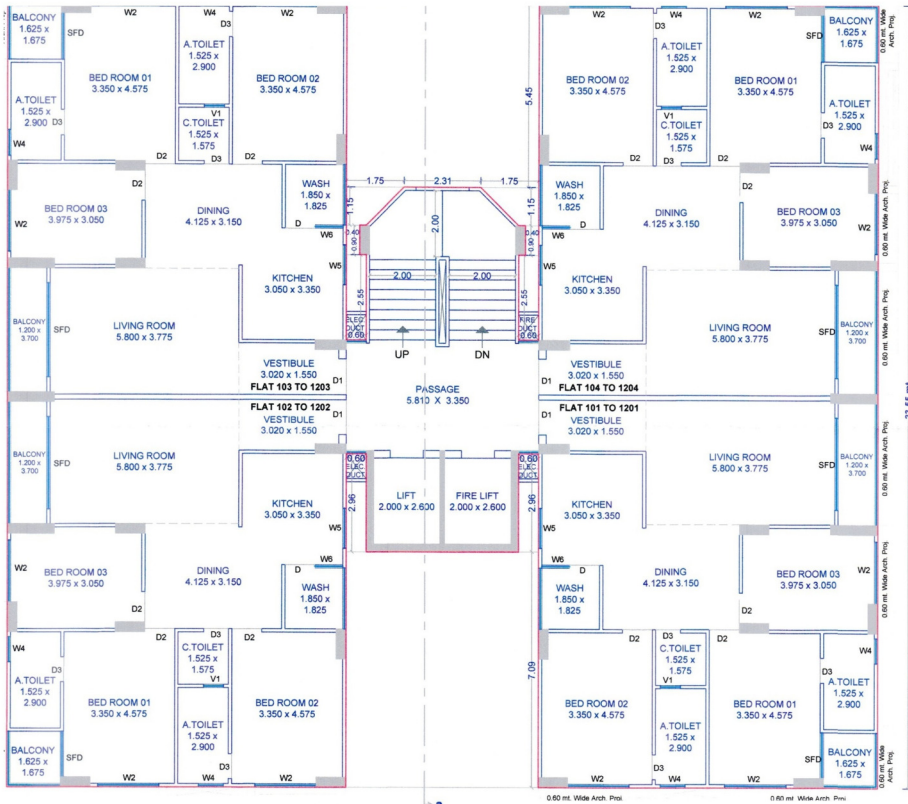
TYPICAL FLOOR PLAN (1ST TO 12TH)
