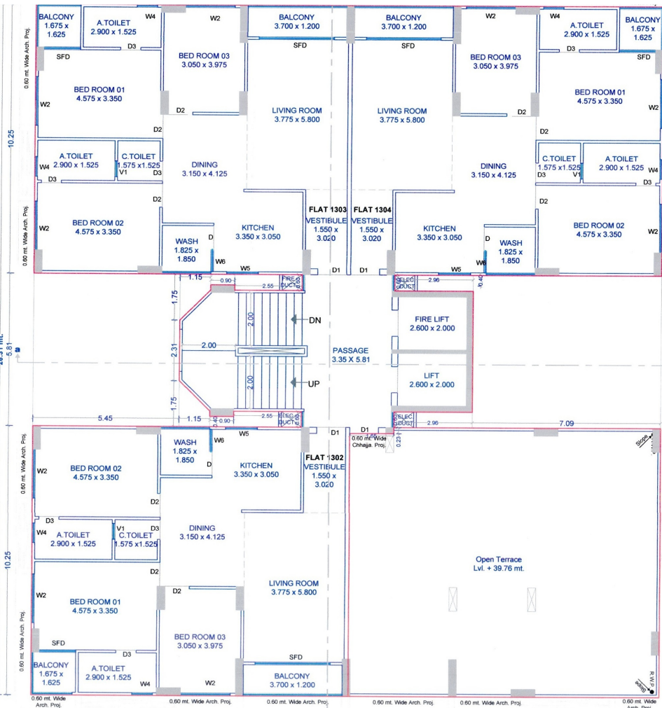
13TH FLOOR PLAN
