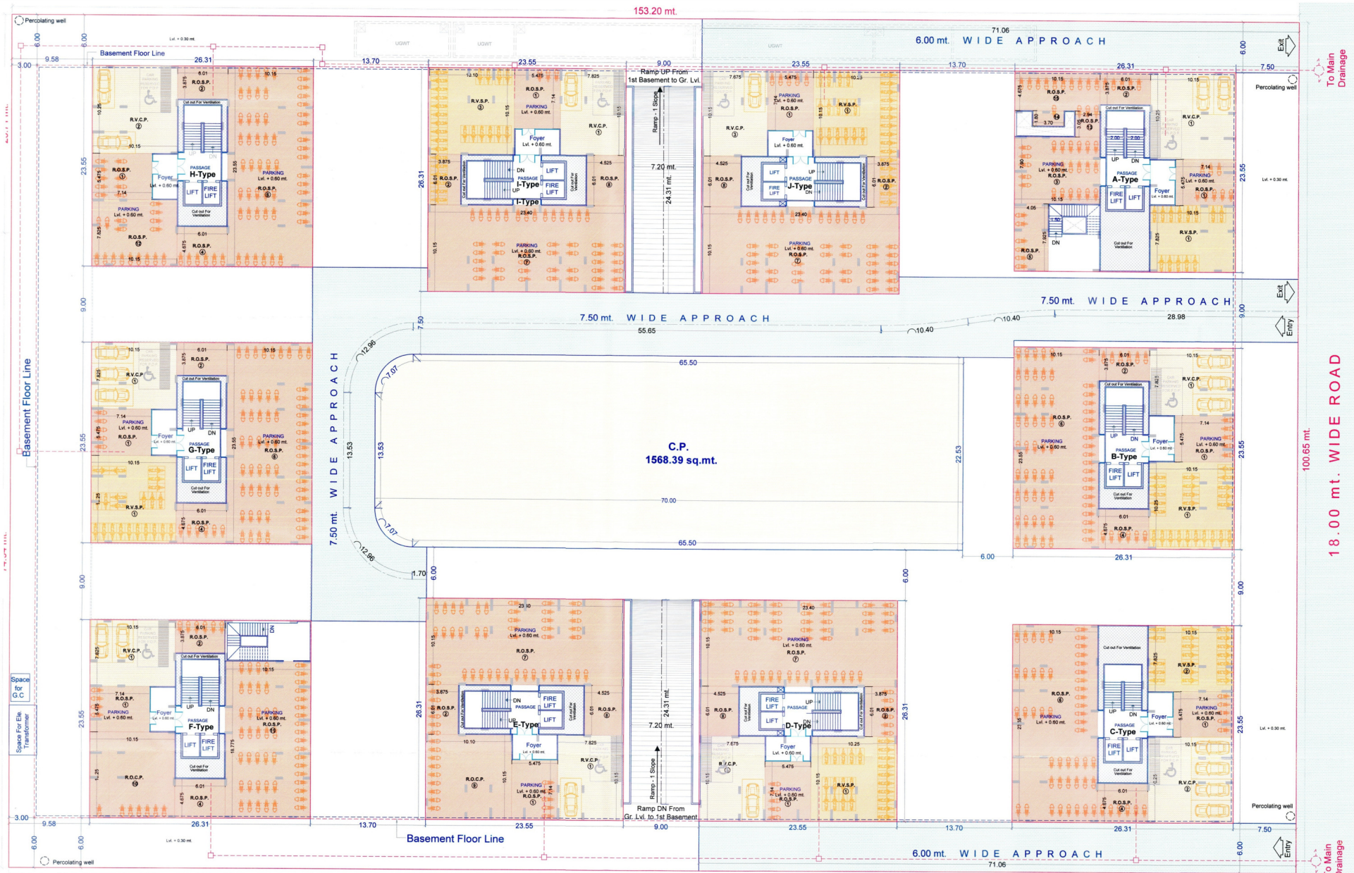
GROUND FLOOR PARKING LAYOUT PLAN
