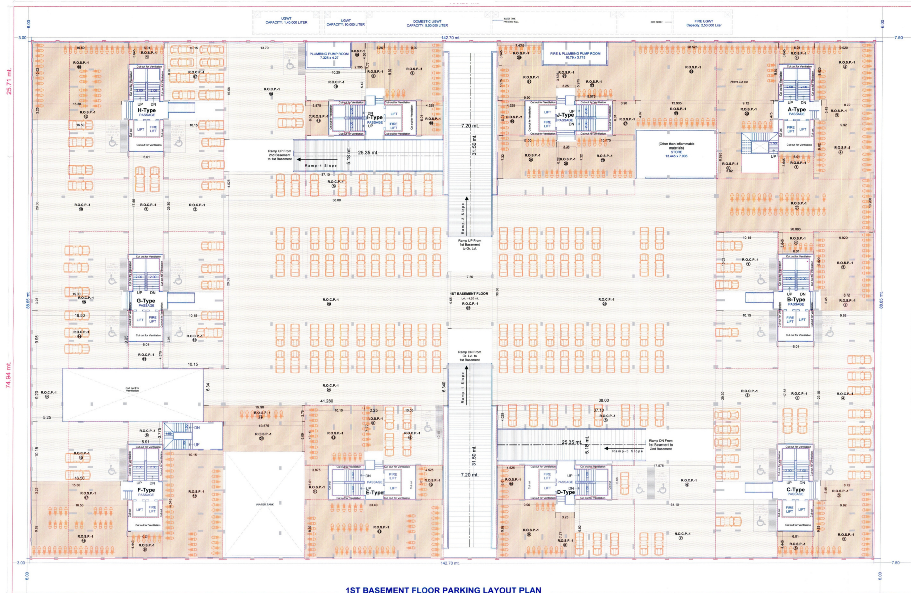
1ST BASEMENT FLOOR PARKING LAYOUT PLAN 153.20 mt.
