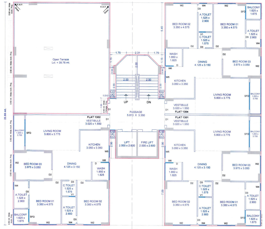
13TH FLOOR PLAN Lvl. +39.76 mt.
