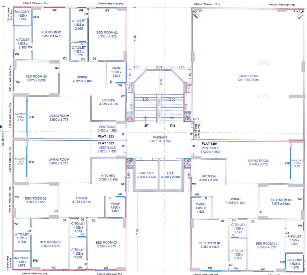
13TH FLOOR PLAN
