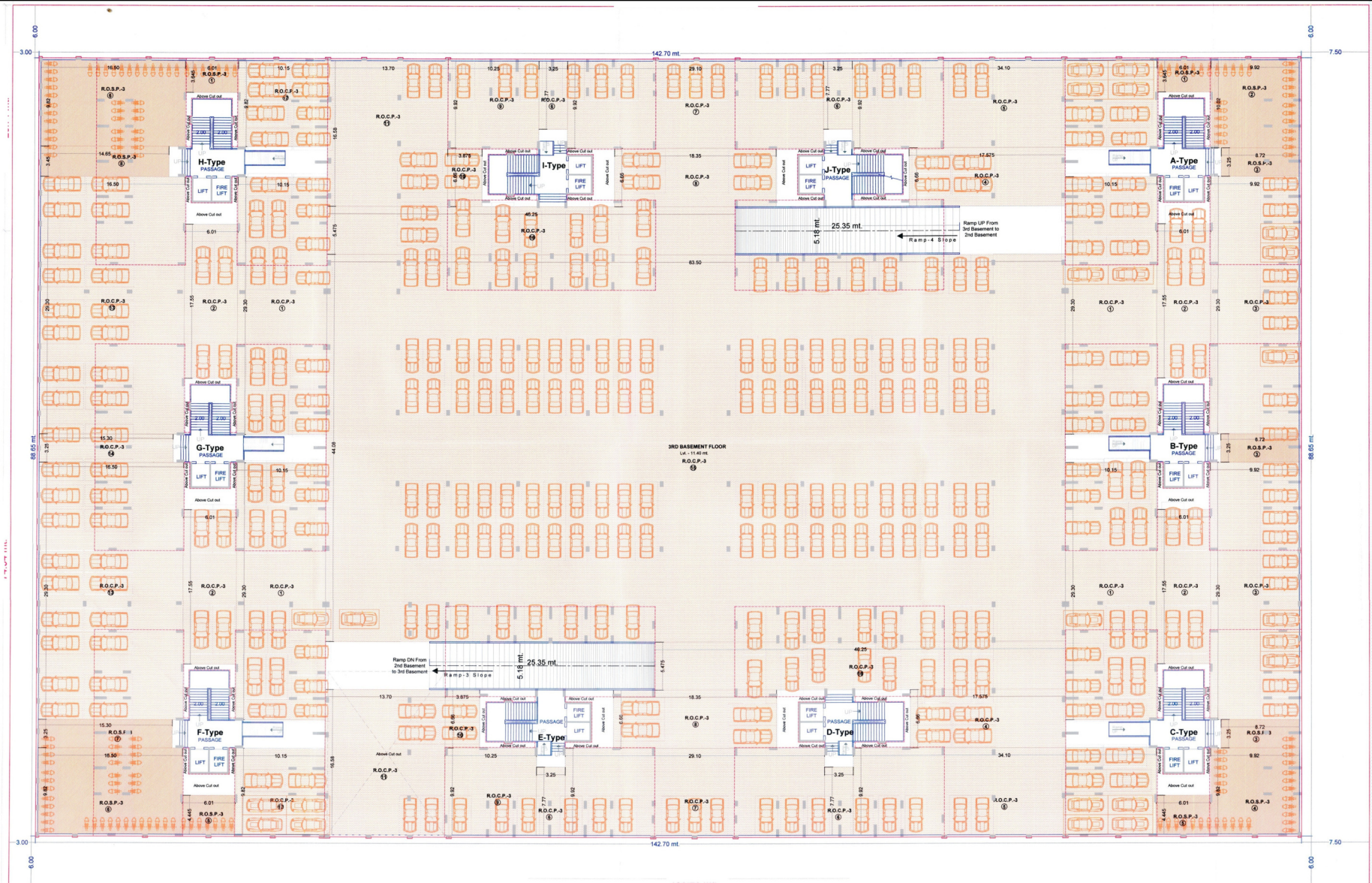
3RD BASEMENT FLOOR PARKING LAYOUT PLAN
