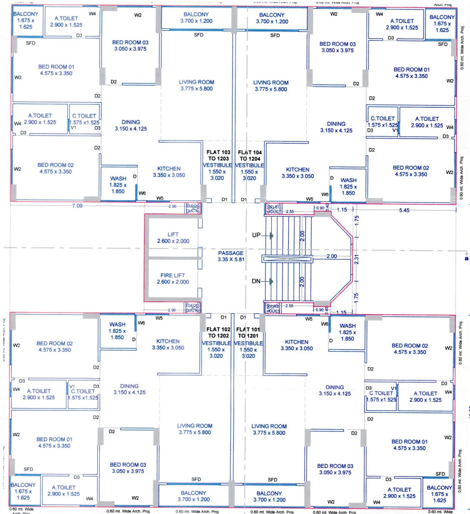
TYPICAL FLOOR PLAN (1ST TO 12TH)
