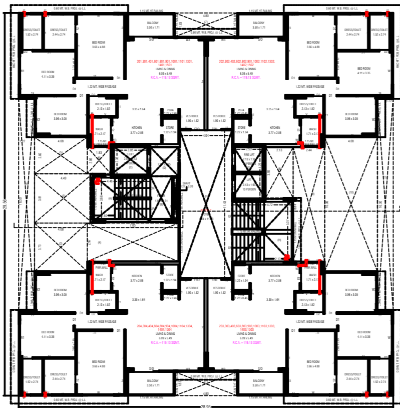
2ND, TO 4TH, 6TH, 8TH, TO 11TH, 13TH, TO 15TH FL. PLAN
