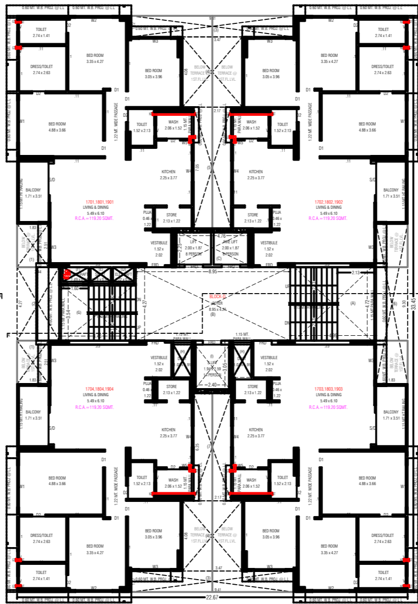
17TH. TO 19TH.FL.PLAN
