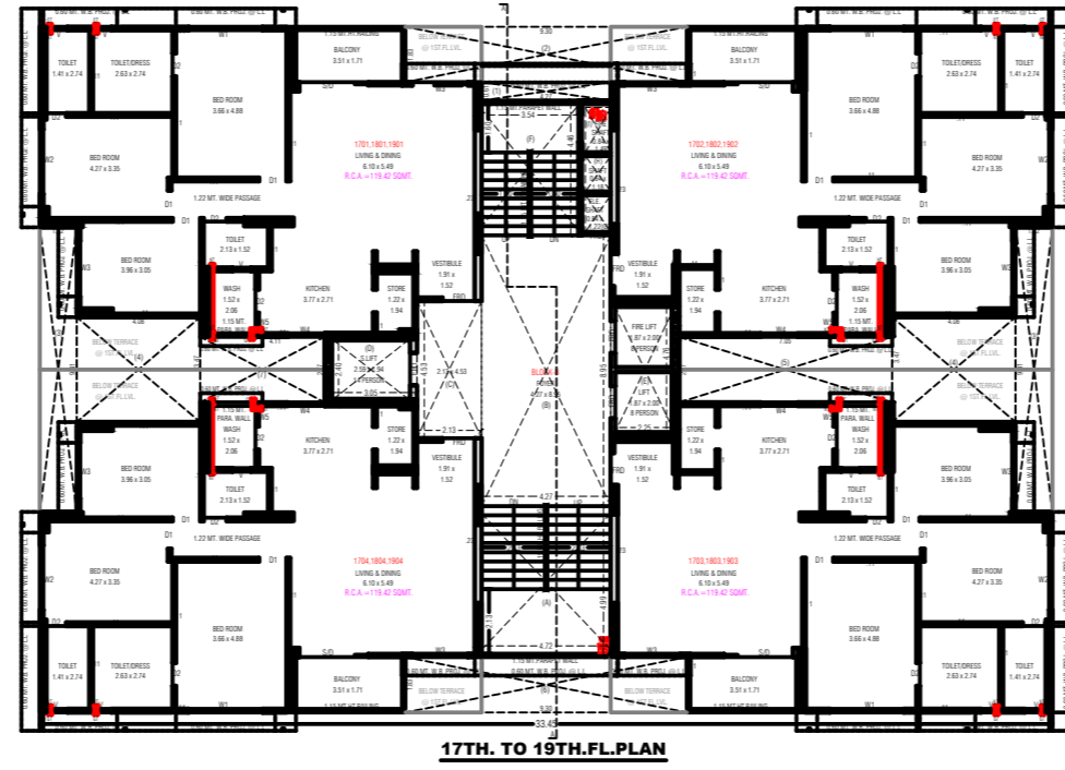
17TH. TO 19TH.FL.PLAN
