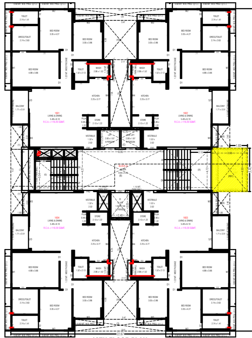
16TH.FLOOR PLAN
