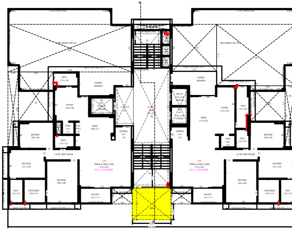
21ST.FLOOR PLAN
