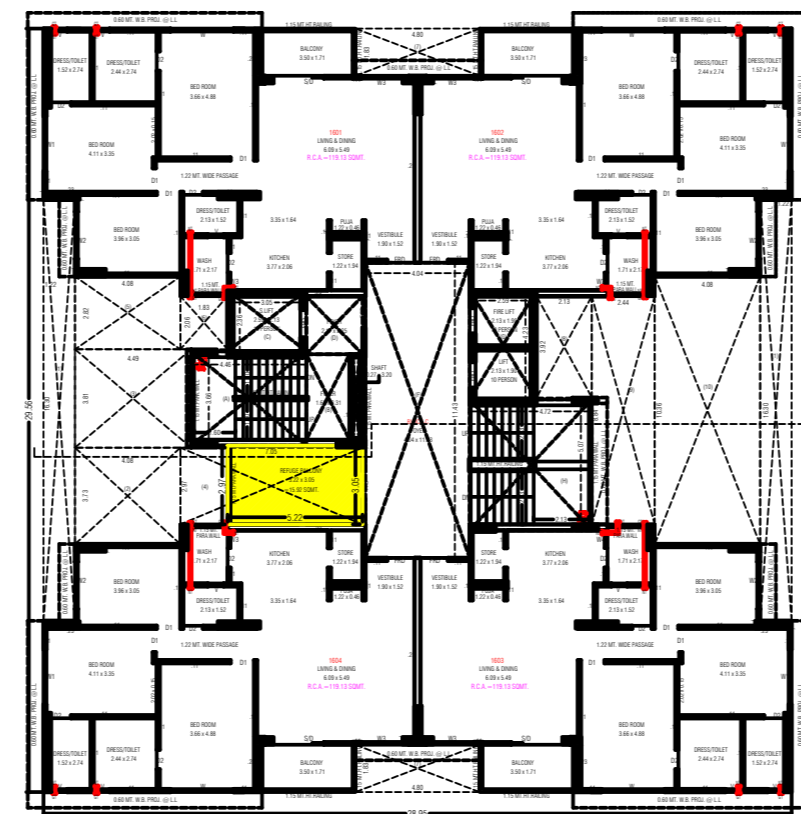
16TH FLOOR PLAN
