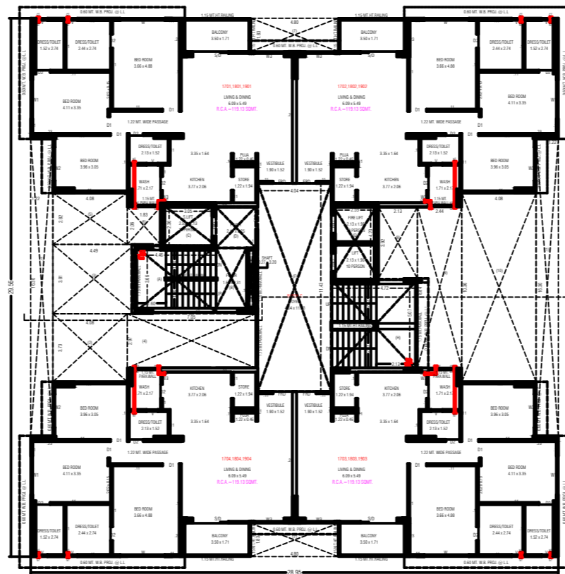
17TH, TO 19TH FL. PLAN
