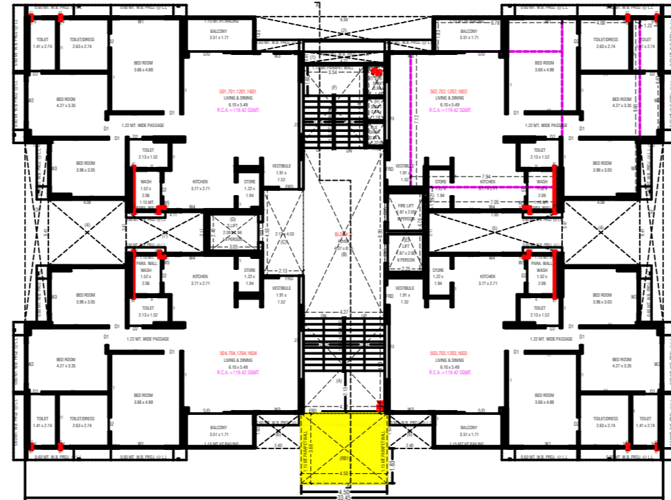
16TH.FLOOR PLAN
