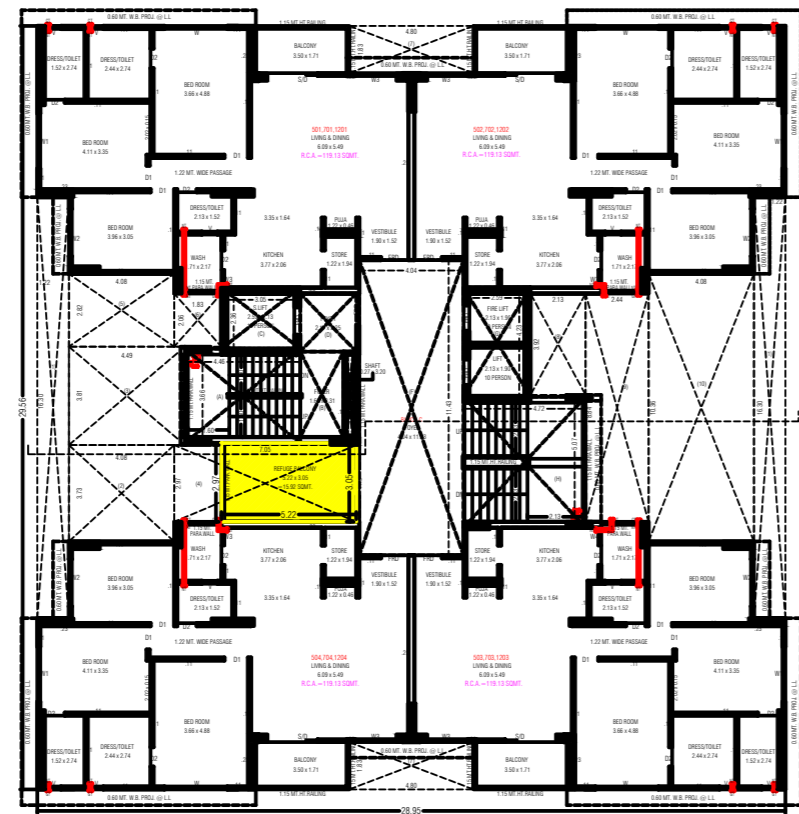
5TH, 7TH, 12TH FLOOR PLAN
