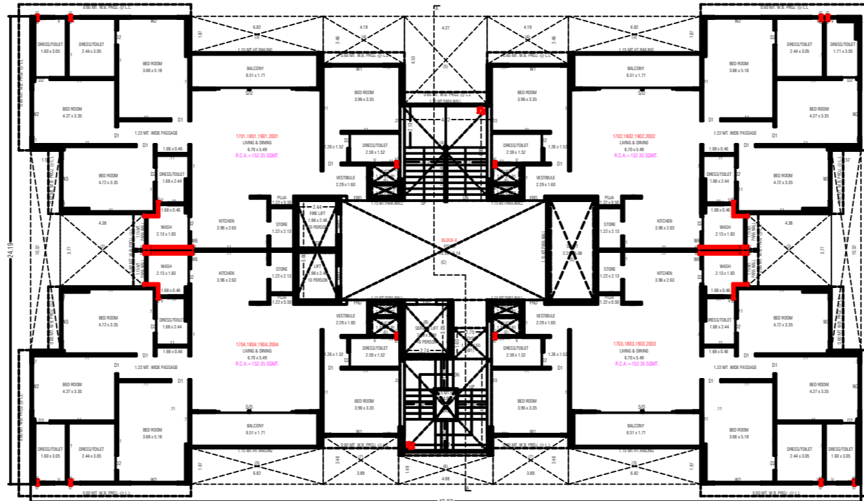
17TH. TO 20TH.FL.PLAN
