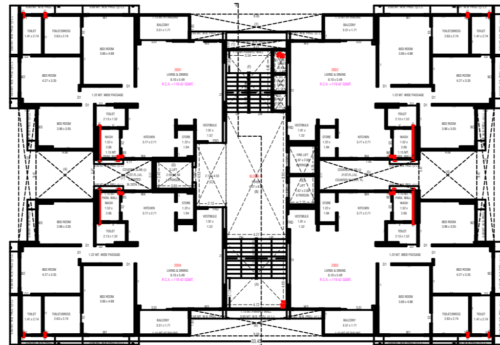
20TH.FLOOR PLAN
