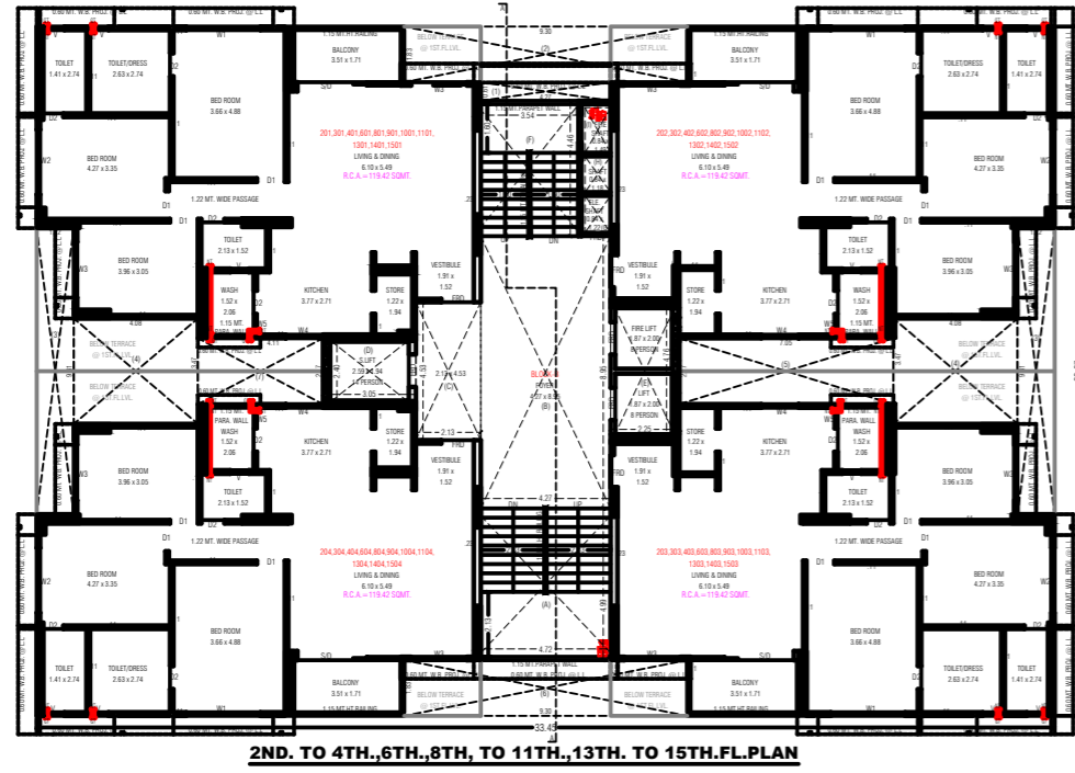
2ND. TO 4TH., 6TH., 8TH., TO 11TH., 13TH. TO 15TH.FL.PLAN
