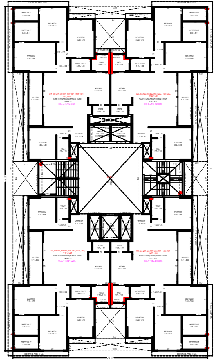
2ND. TO 4TH., 6TH., 8TH. TO 11TH., 13TH. TO 15TH. FL. PLAN
