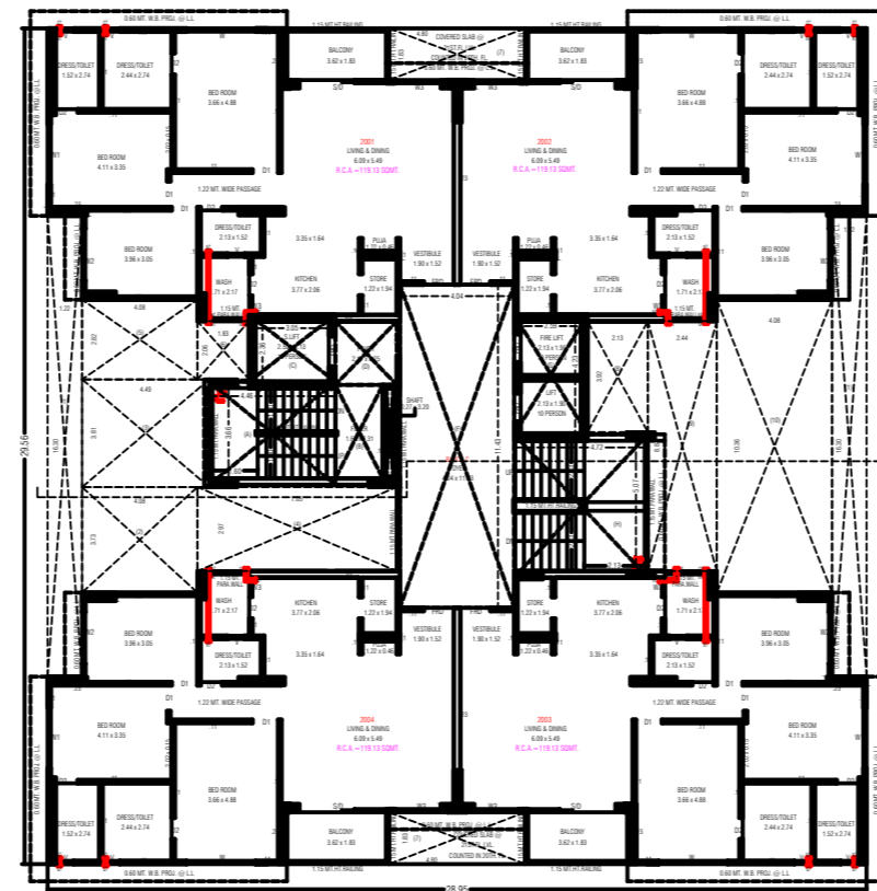
20TH FLOOR PLAN
