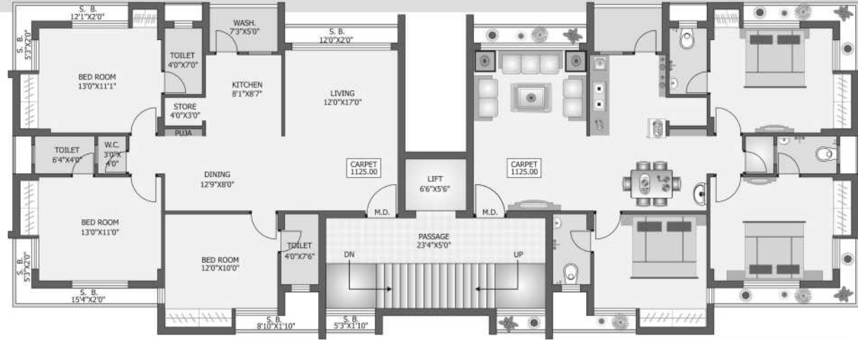
Typical 1st to 5th FLOOR PLAN
