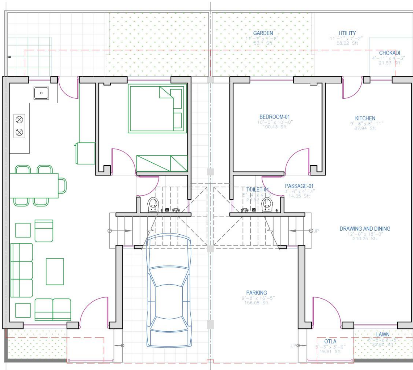
TYPE A CARPET AREA 142.155 sq. mt. GROUND FLOOR PLAN
