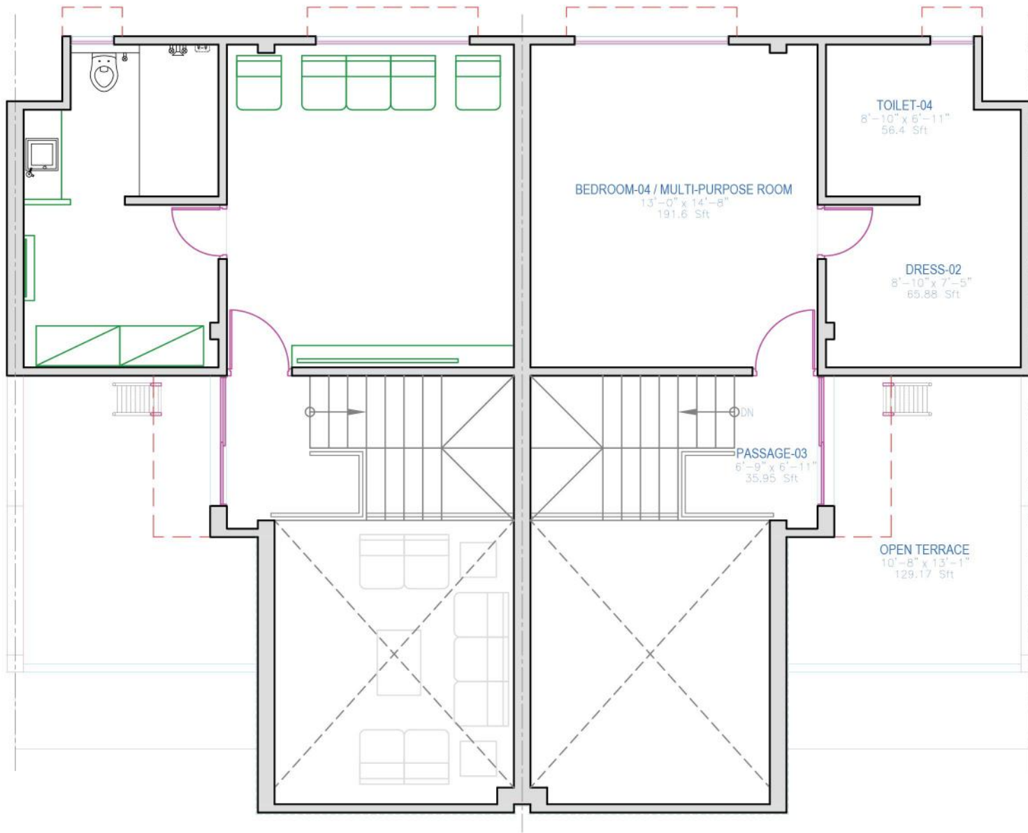
TYPE A CARPET AREA 142.155 sq. mt. SECOND FLOOR PLAN
