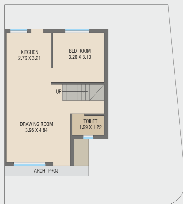
BLOCK NO.28 GROUND FLOOR PLAN B-UP AREA : 52.59 SQ.MT.
