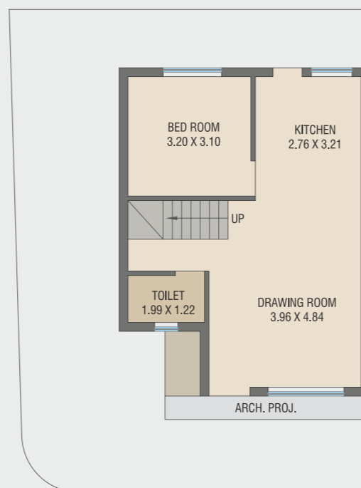
BLOCK NO.87 GROUND FLOOR PLAN B-UP AREA : 52.59 SQ.MT.
