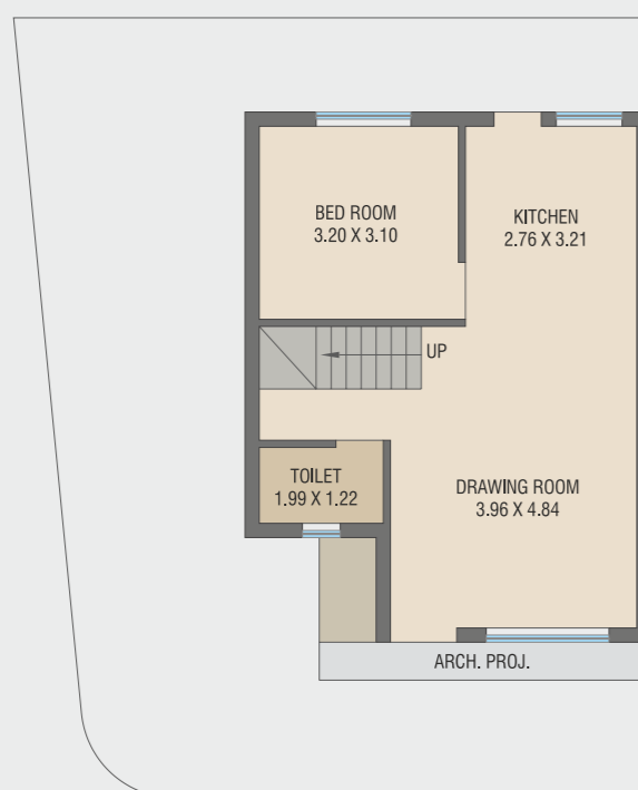
BLOCK NO.13 GROUND FLOOR PLAN B-UP AREA : 52.59 SQ.MT.
