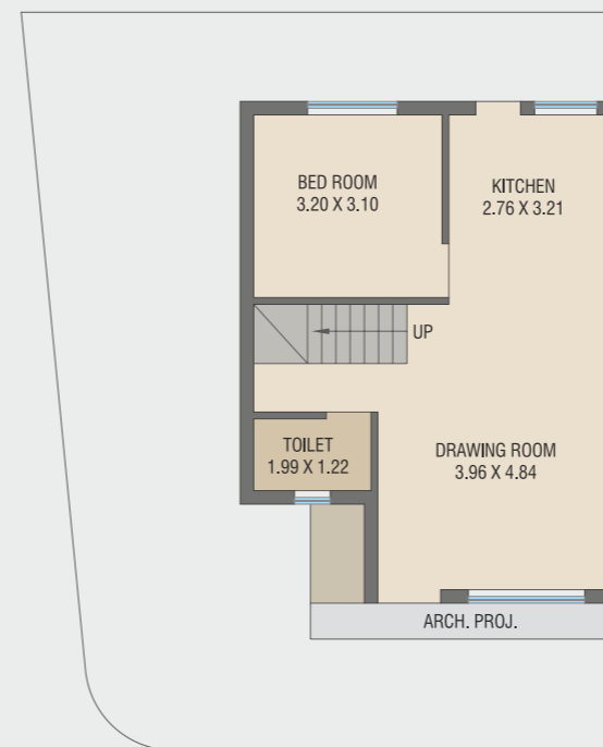
BLOCK NO.29 GROUND FLOOR PLAN B-UP AREA : 52.59 SQ.MT.
