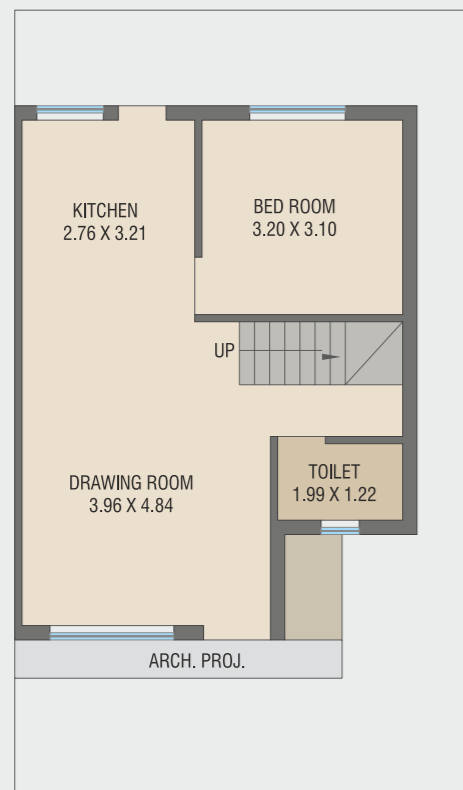
BLOCK NO.135 TO 138 GROUND FLOOR PLAN B-UP AREA : 52.59 SQ.MT.
