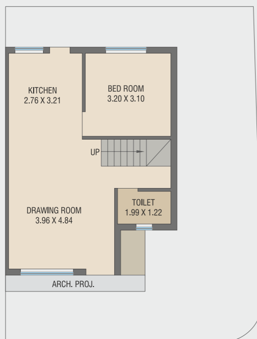
BLOCK NO.86 GROUND FLOOR PLAN B-UP AREA : 52.59 SQ.MT.
