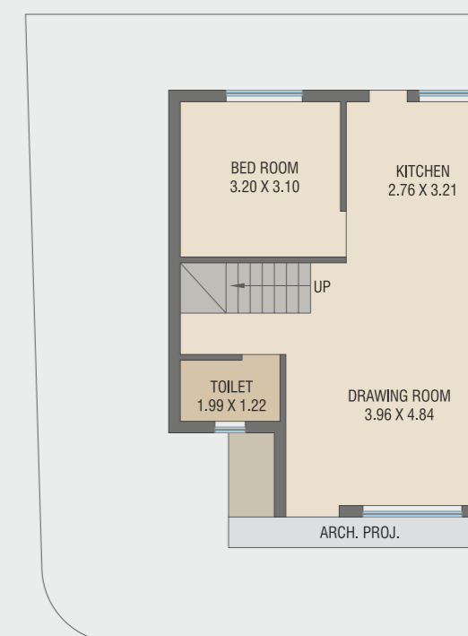
BLOCK NO.58 GROUND FLOOR PLAN B-UP AREA : 52.59 SQ.MT.
