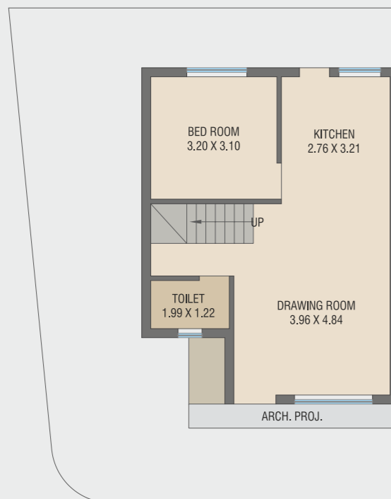
BLOCK NO. 01 GROUND FLOOR PLAN B-UP AREA : 52.59 SQ.MT.
