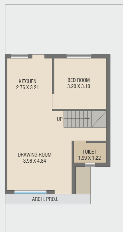
BLOCK NO.118 TO 124, 126 TO 134 GROUND FLOOR PLAN B-UP AREA : 52.59 SQ.MT.
