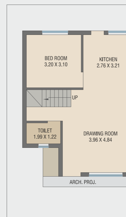
BLOCK NO. GROUND FLOOR PLAN B-UP AREA : 52.59 SQ.MT.
