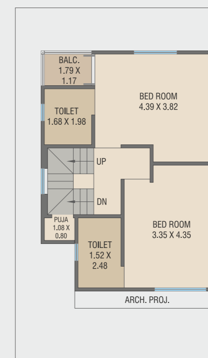
BLOCK NO. FIRST FLOOR PLAN B-UP AREA : 52.59 SQ.MT.
