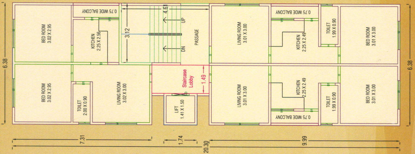
TYPICAL - 1-4 FLOOR PLAN
