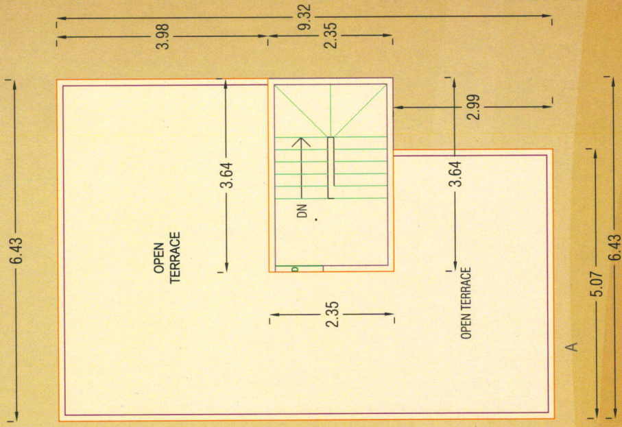
TERRACE (CABIN) FLOOR PLAN
