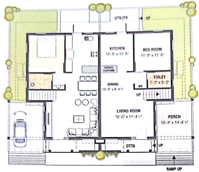
Ground Floor Plan Carpet Area : 600.83 Sq. Ft. S. B. Area : 1090.89 Sq. Ft.
