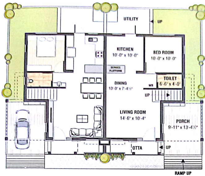
Ground Floor Plan Carpet Area : 500.35 Sq. Ft. S. B. Area : 823.69 Sq. Ft.
