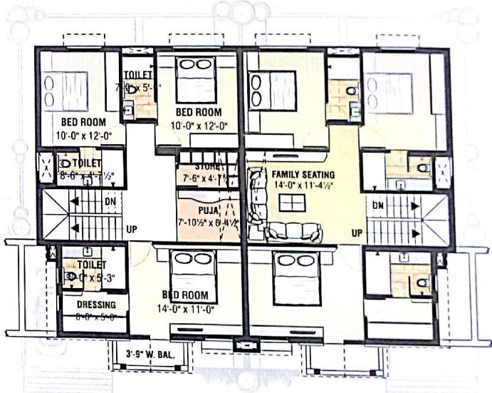
First Floor Plan Carpet Area : 821.59 Sq. Ft. S. B. Area : 942.88 Sq. Ft.
