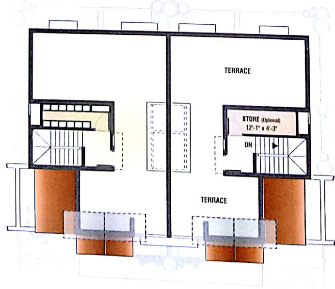
First Floor Plan Carpet Area : 821.59 Sq. Ft. S. B. Area : 942.88 Sq. Ft.
