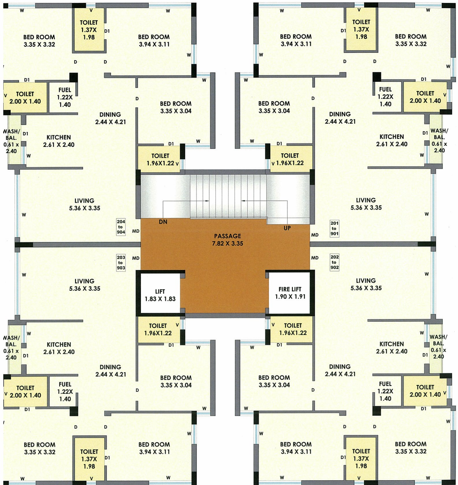
2ND TO 9TH FLOOR PLAN (TOWER - "A")
