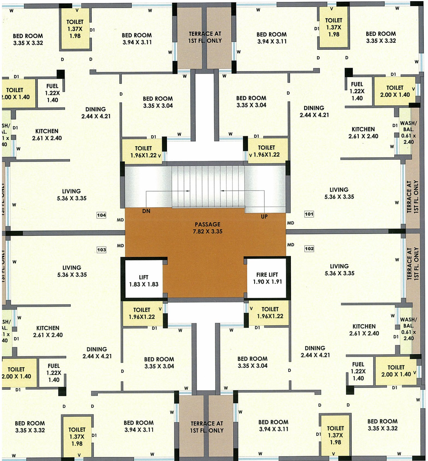
1ST FLOOR PLAN (TOWER - "A")
