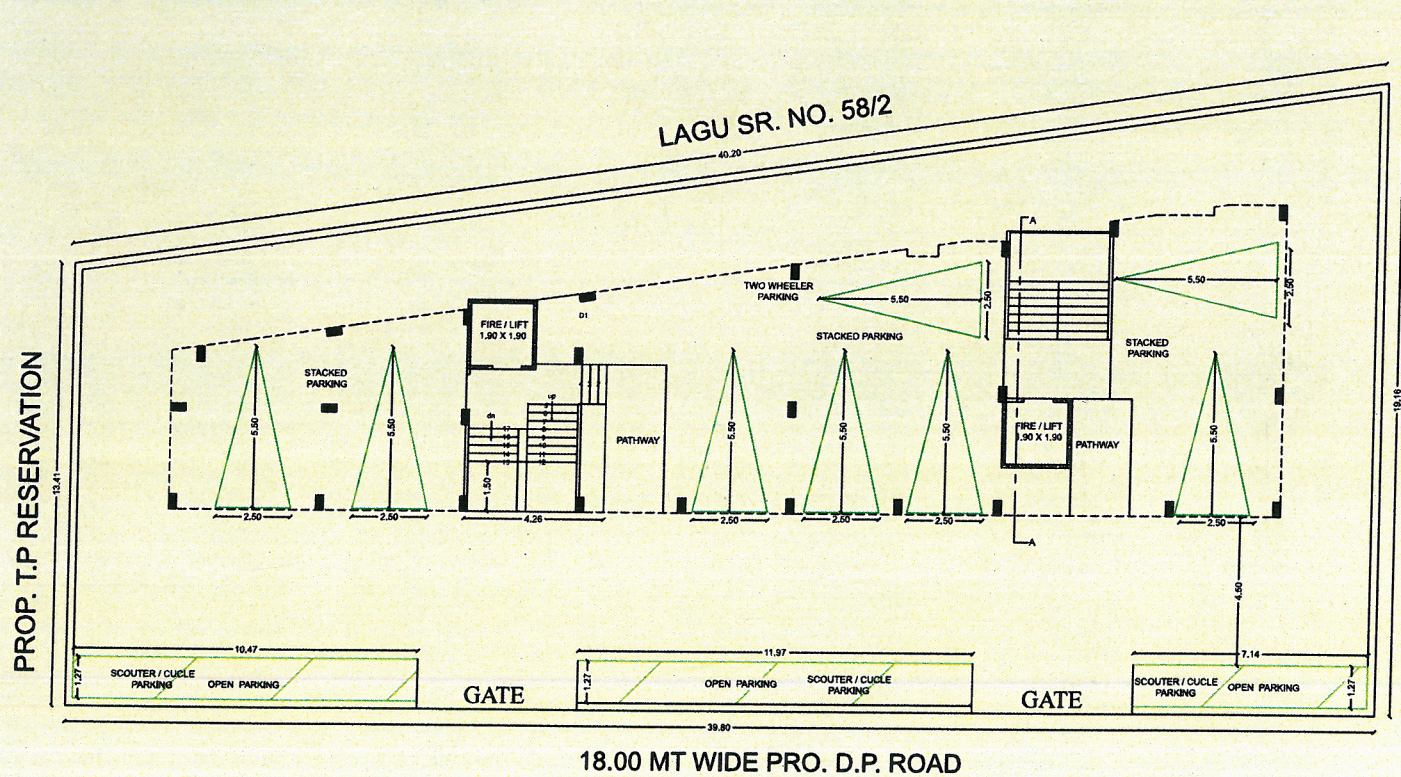
CELLAR PARKING PLAN
