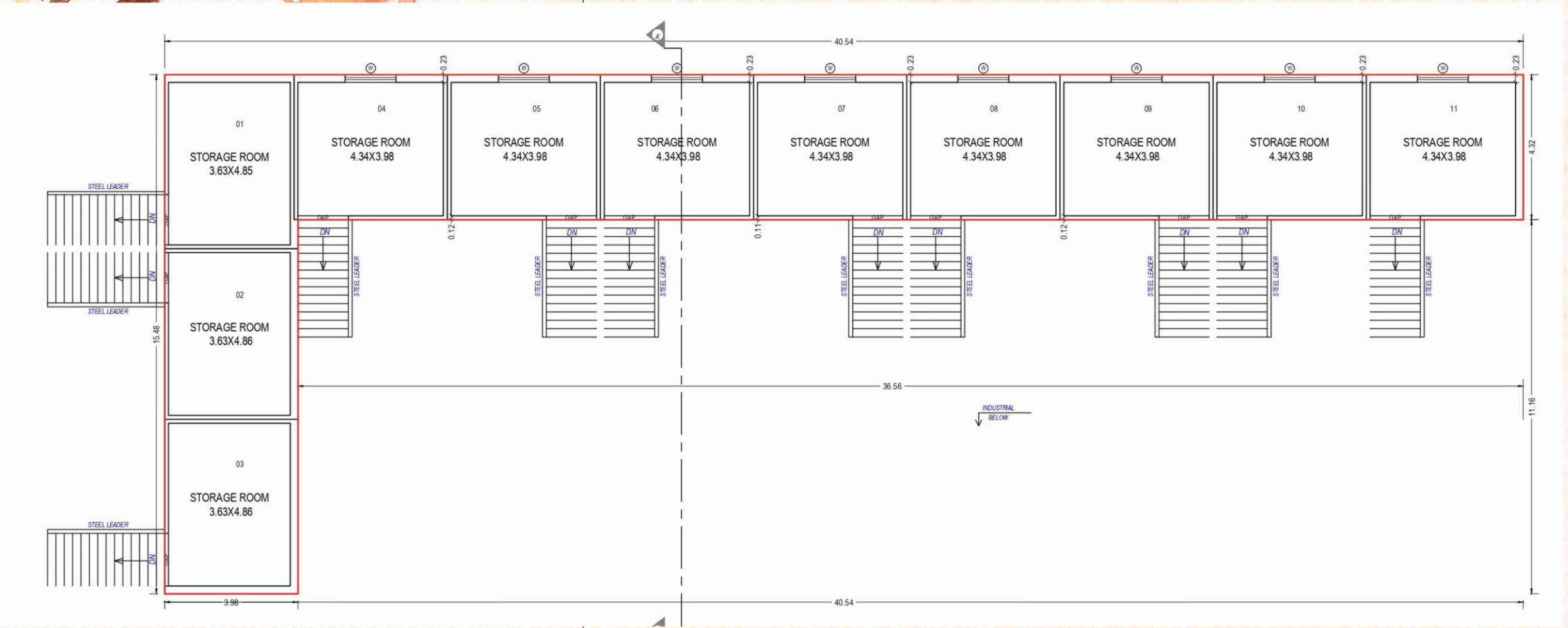
MEZZANINE FLOOR PLAN
