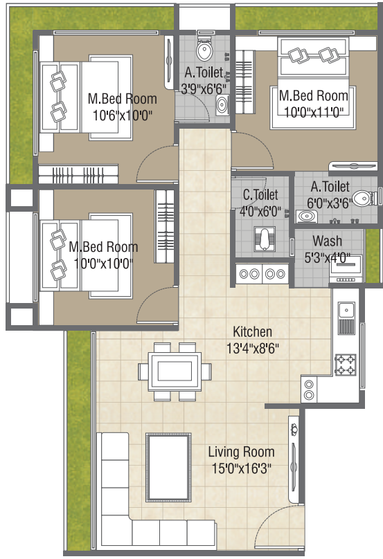
3 BHK TYPICAL FLOOR PLAN (1 st to 14 th Floor Building - B)
