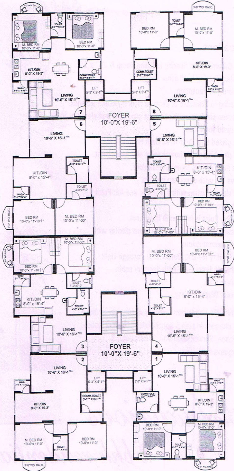
Typical Plan
