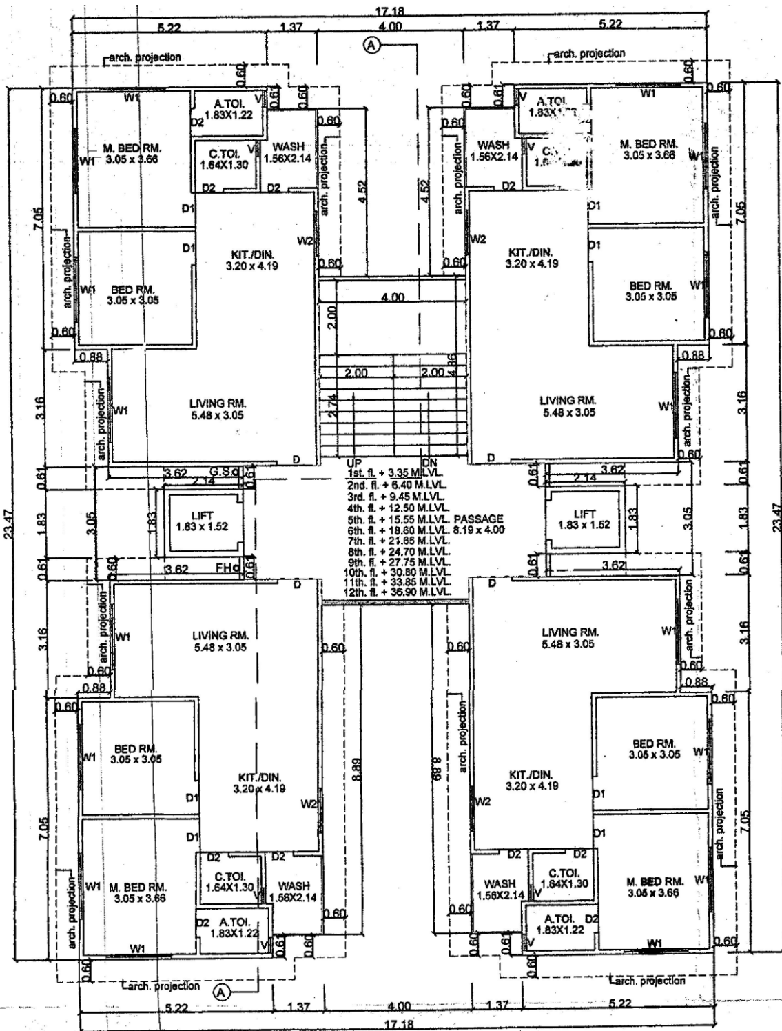
TYPICAL (1ST. TO 12TH.) FLOOR PLAN SCALE 1 CM. = 1 MT.
