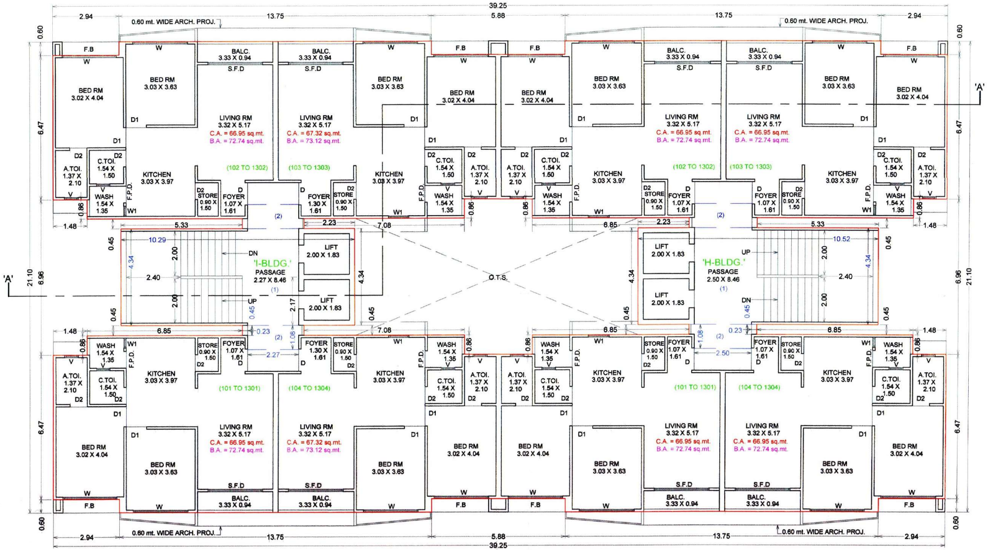
1st. TO 13th.FLOOR PLAN (LVL. +4.30 mt. TO LVL. +39.10 mt.)
