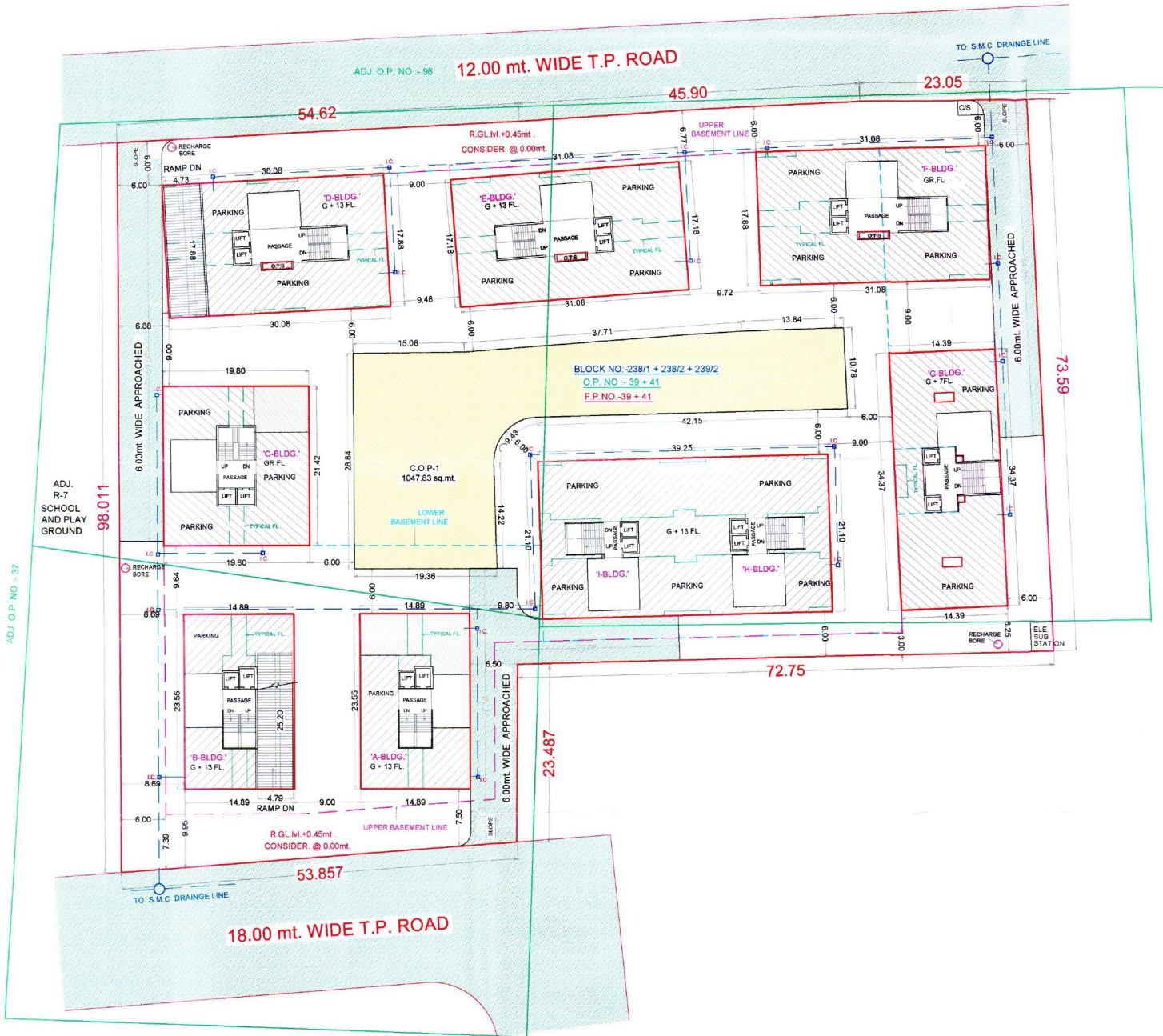
LAY OUT PLAN (SCALE = 1cm = 4.0 mt.)
