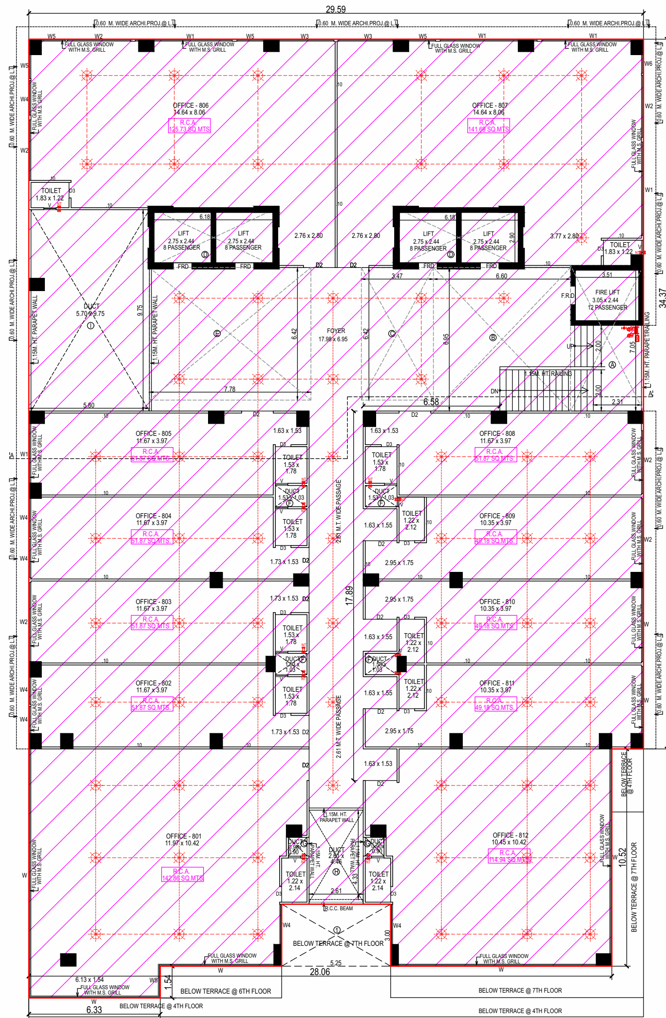
8TH FLOOR PLAN
