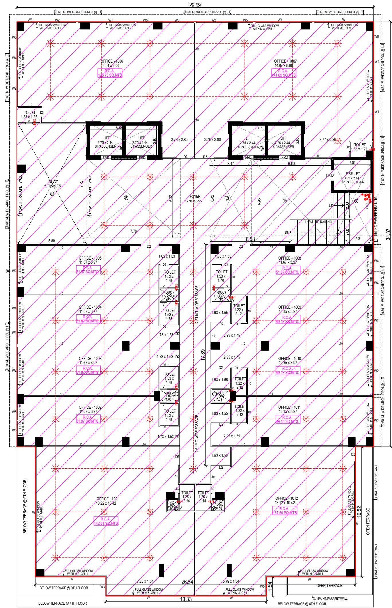
10TH FLOOR PLAN
