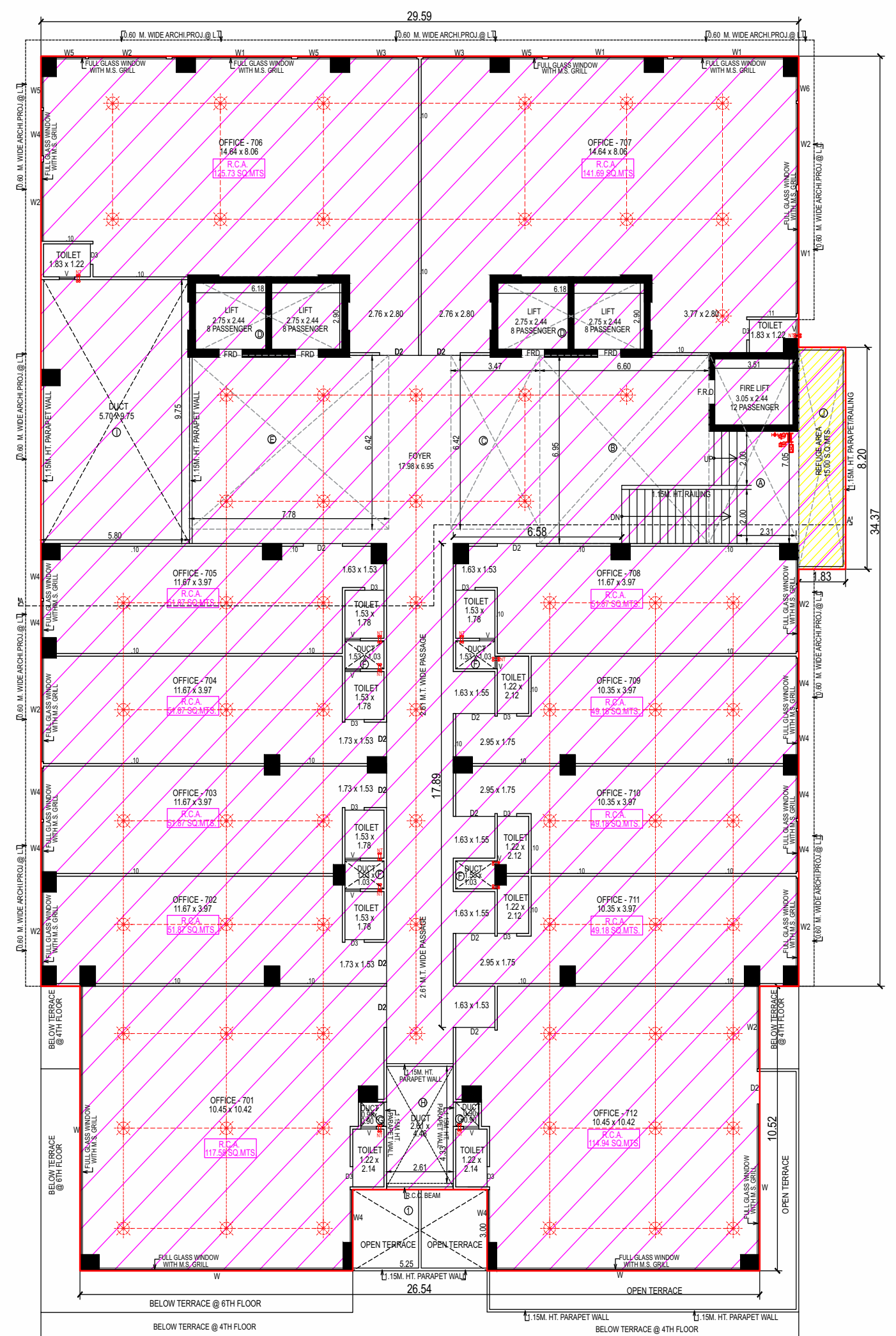
7TH FLOOR PLAN
