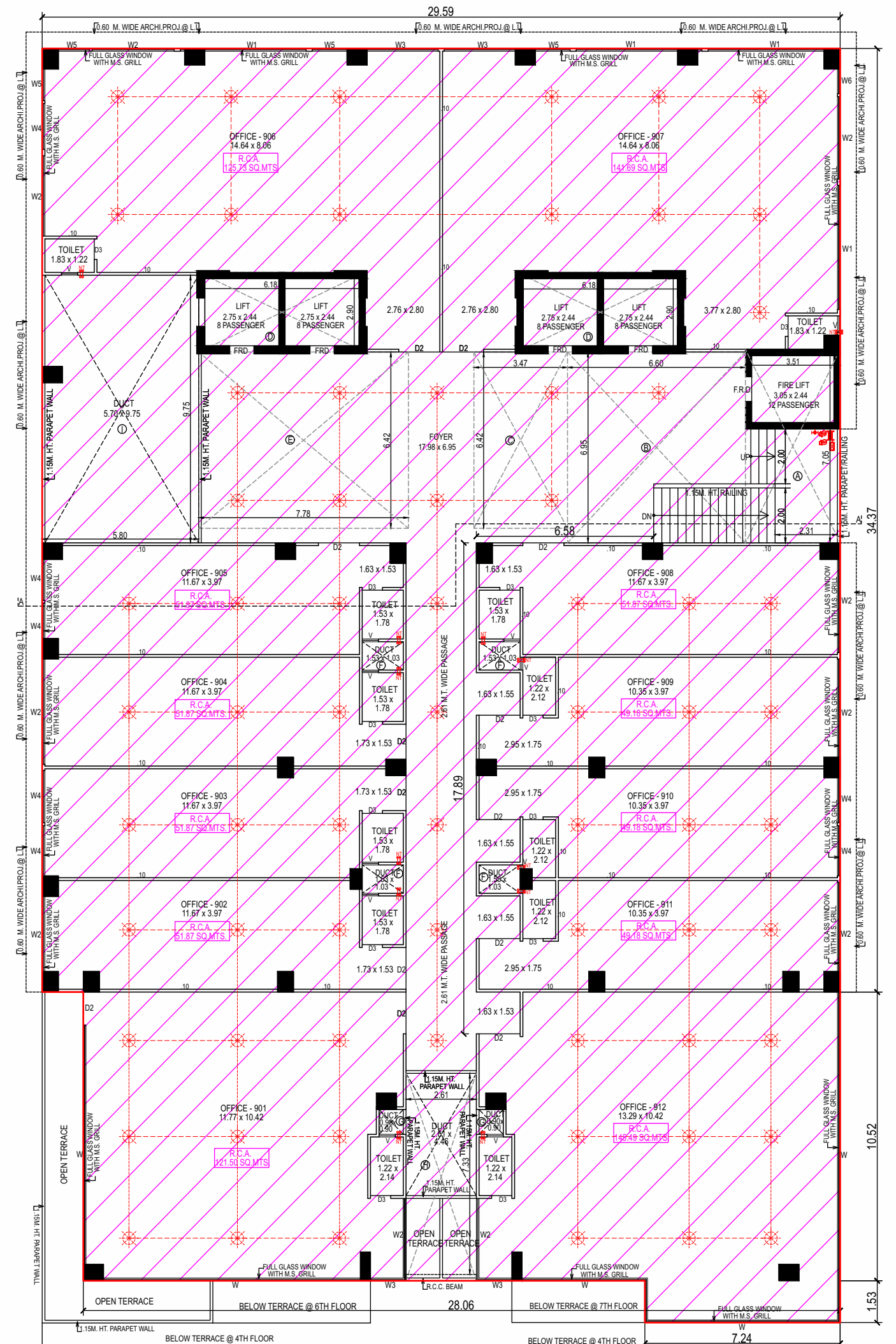
9TH FLOOR PLAN
