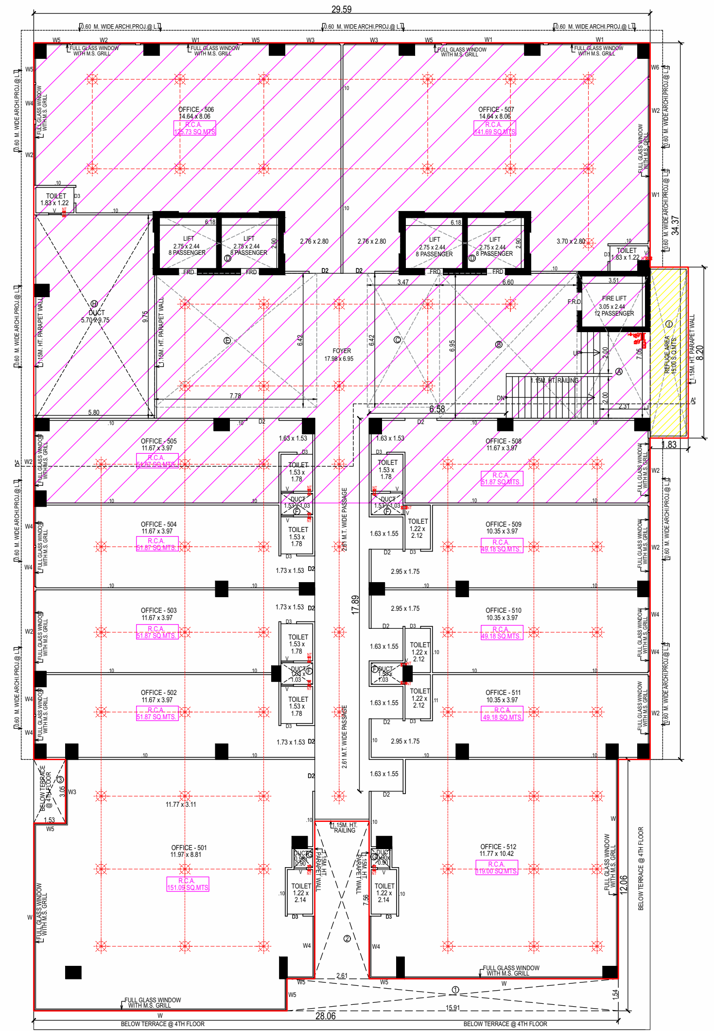
5TH FLOOR PLAN
